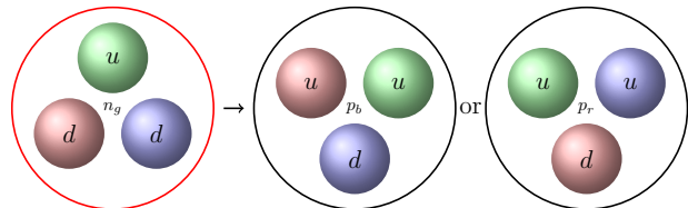
Fig. 3.1 Neutron to Proton transformation
