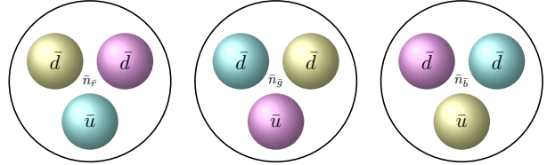
Fig. 2.2 The three types of antineutrons
