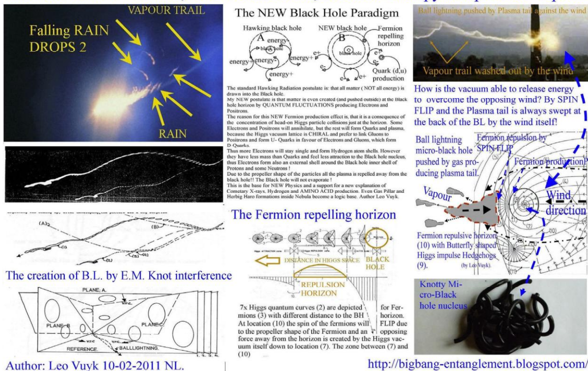
Figure: 15, The start of my research was: Ball Lightning physics. Such as Quantum Knot-interference BLs and the origin of acceleration of Knotty BL micro black holes (Quantum Knots) by pushing plasma tails.
