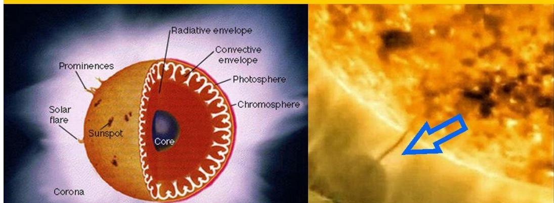
Figure: 17, ( see also ref. [13]) Bright points or spots at the solar surface represent small Comets able to leave the sun by new pushing Cometary tails like Ball Lightnings do. The origin of these bright points are supposed to be so called “Interference black holes” according to Q-FFF theory.
