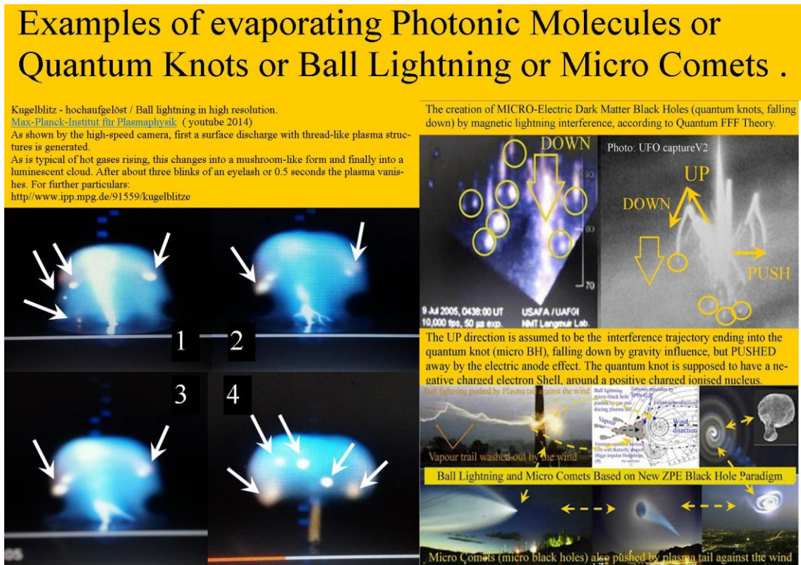
Figure 7, examples of evaporating micro Black Holes also called Photonic Molecules, Quantum Knots, Ball Lightning or even Micro Comets.
