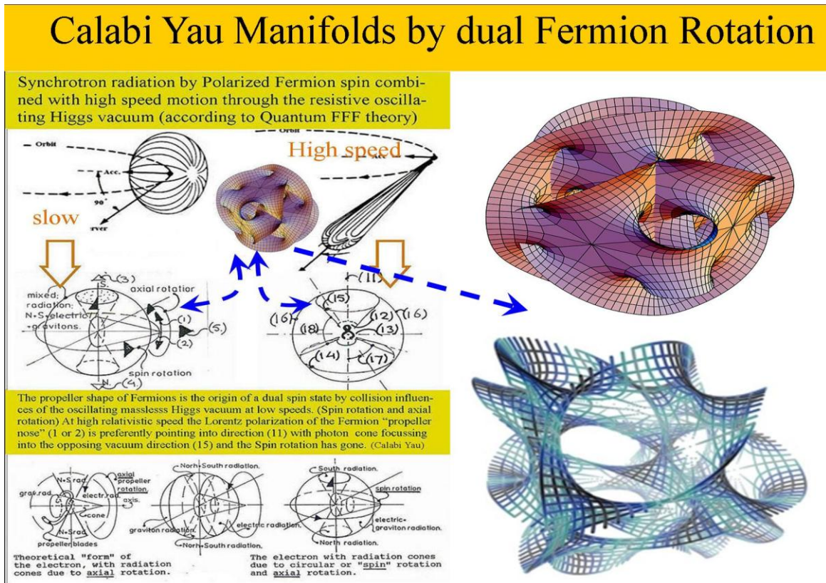
Figure 25. Calabi Yau Manifolds.
