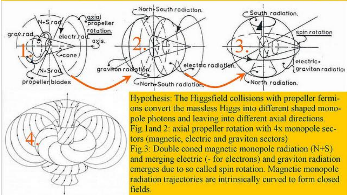
Figure: 3. Fermion spin related radiation sector diagrams according to Quantum FFF Theory. Related to Penrose proposal
