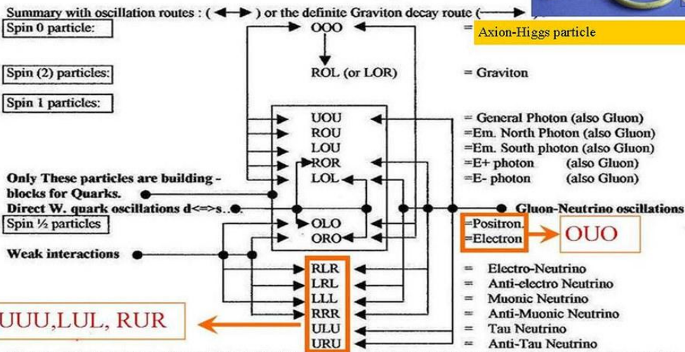
Figure 20, Alternative Feynman diagrams presenting all forces in nature. In combination with the particle zoo of single ELEMENTARY particles made out of ONE convertible Torus shaped Axion/ Higgs particle, equipped with three hinges of 90 degree rotation.
