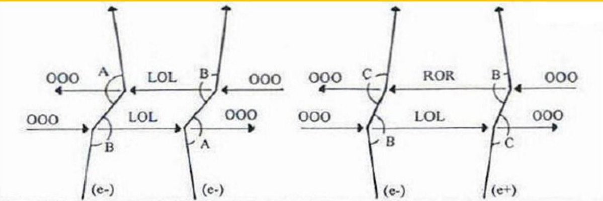
(Above) Alternative Feynman diagrams for electron-positron attraction and electron-electron repulsion by Dipole Repeller system.
