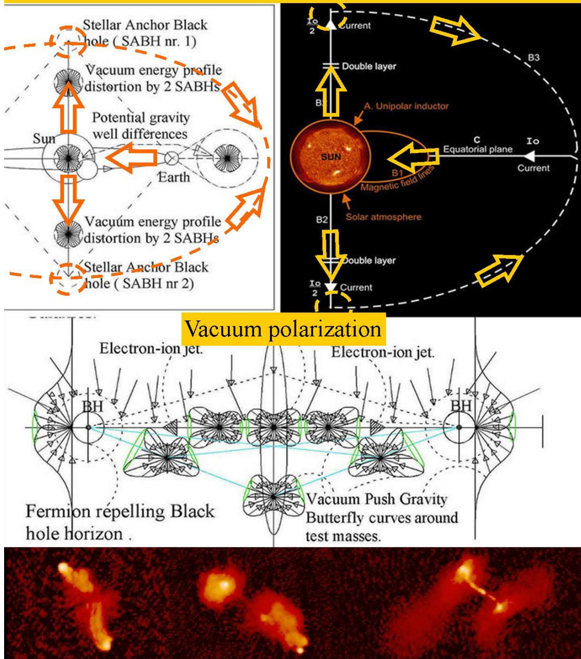
Figure: 17, Black hole propulsion and pairing principle of fig 15, seems to be the origin of dual Stellar or galaxy Anchor black holes (see figure 19) and even so called Birkeland /Alfvén current circuits around stars and galaxies by vacuum polarization. The energetic polarized vacuum oscillation spectrum is the motor for fast gas and electron transport starting direct after the big bang.
