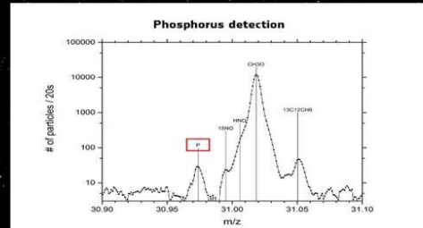
Spectrum indicating phosphorus [P] detection, along with other gases, on 26 October 2014. Phosphorus is a key element in all living organisms. It is found in DNA, RNA and in cell membranes, and it is used in transporting chemical energy within cells for metabolism.
