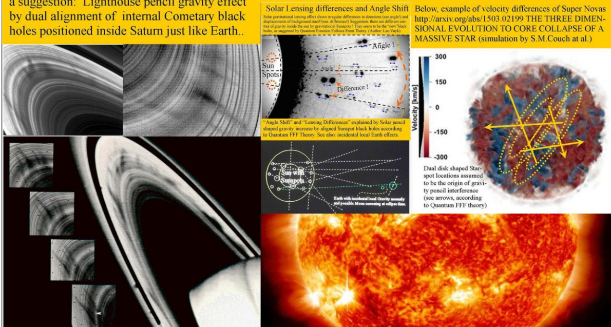
Figure: 4. Pencil shaped gravity wave examples around different objects.
