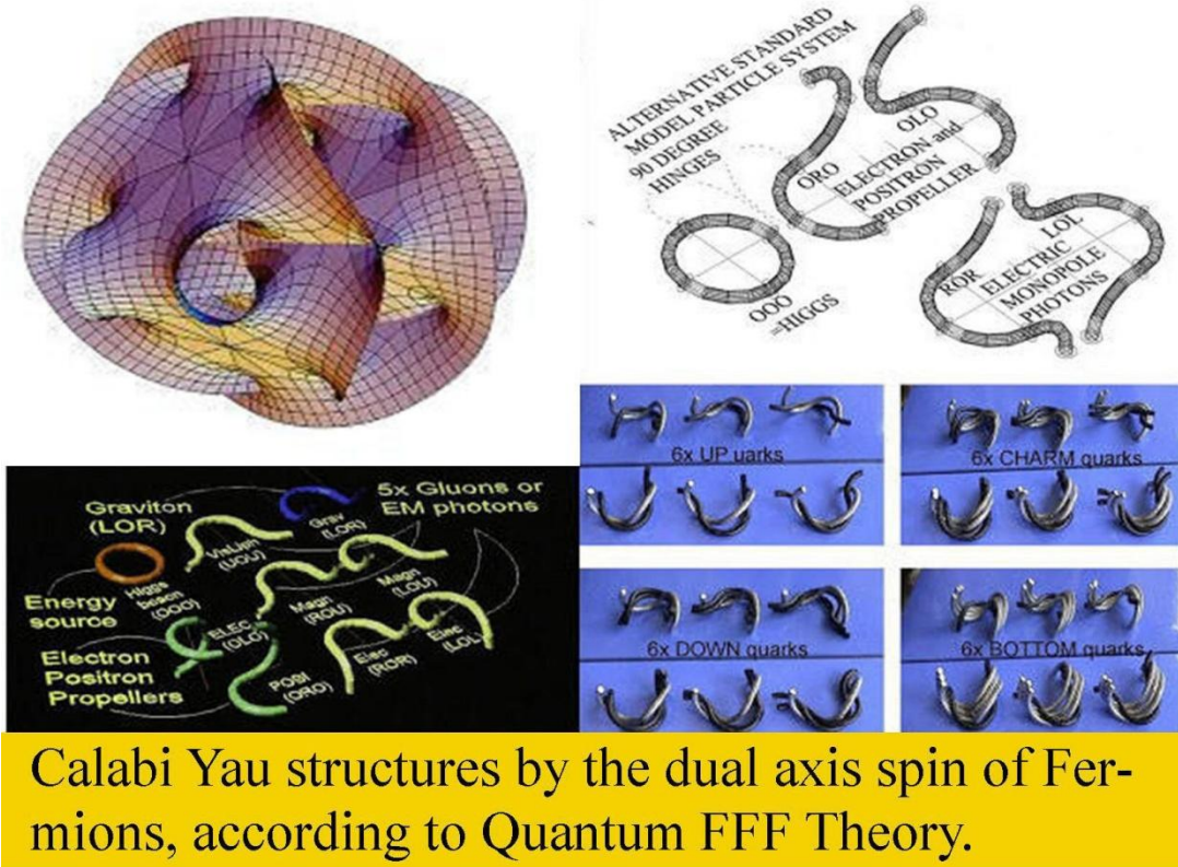
Figure: 6. Cog wheels, joints and hinges at the Quantum scale of spinning Fermion strings with double rotation axis forming Calabi Yau Manifolds.
