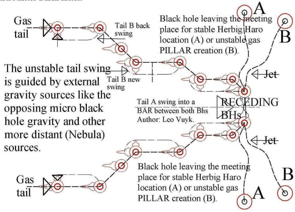
Figure 15, New Black hole propulsion principle by a self produced plasma-dust tail. As a consequence, New micro interference black holes do not merge to form larger nuclei, they even repel negative charged metal surfaces (observed by ball lightning) by their own exterior electron charge.
