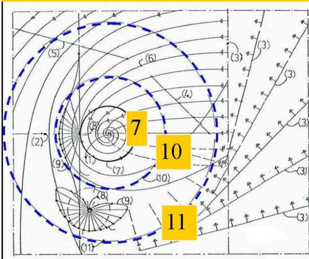
Figure: 25.. Fermion repulsion principle around dark matter black holes producing water ice Comets Megacryometeors. A special example of nuclear water ice production is found in the Moon Hyperion, which is assumed to be a former Comet, left alone by its Black Hole energy source.
