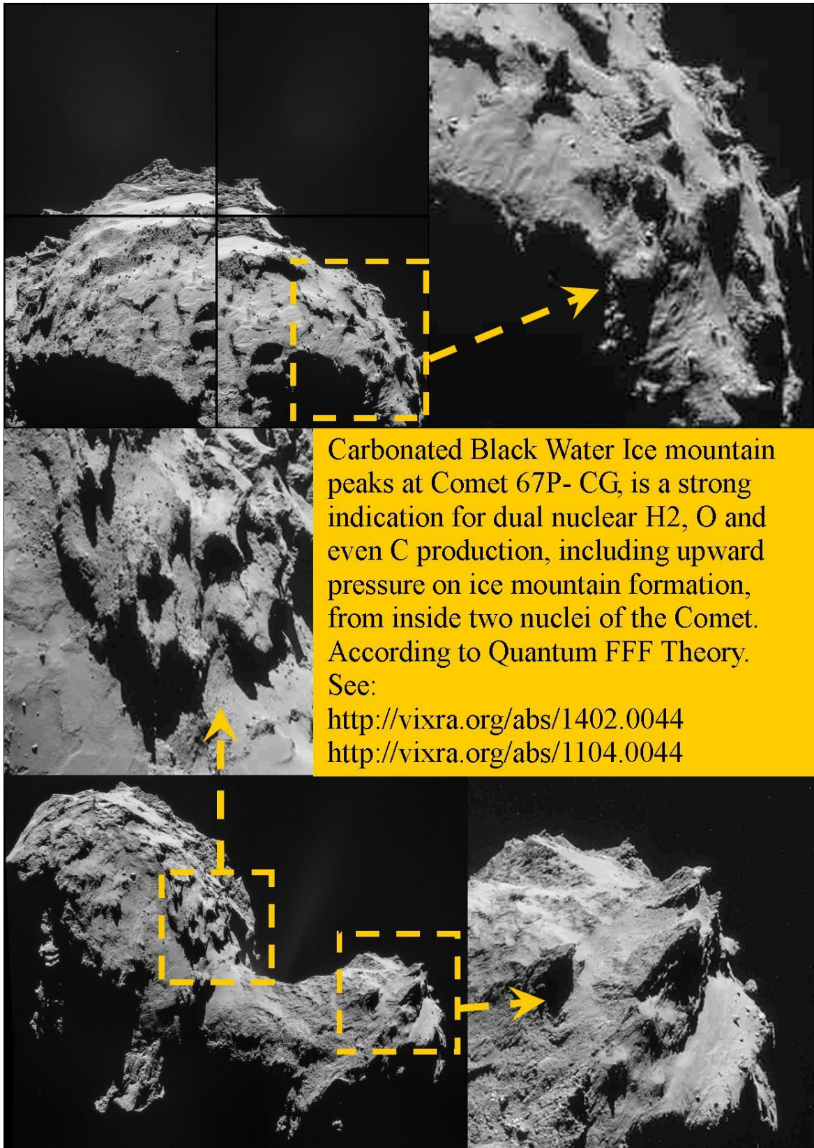
Figure 30, NOT EROSION but Plate tectonics driven by the nuclear matter production of new paradigm dark matter black holes.
