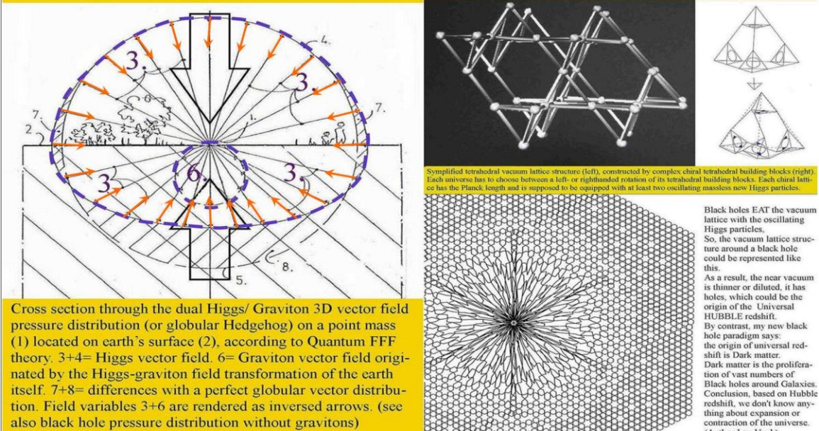
Figure: 12, The massless Axion-Higgs chiral vacuum based on dual oscillating Axion particles inside a a truncated tetrahedral Lattice.
