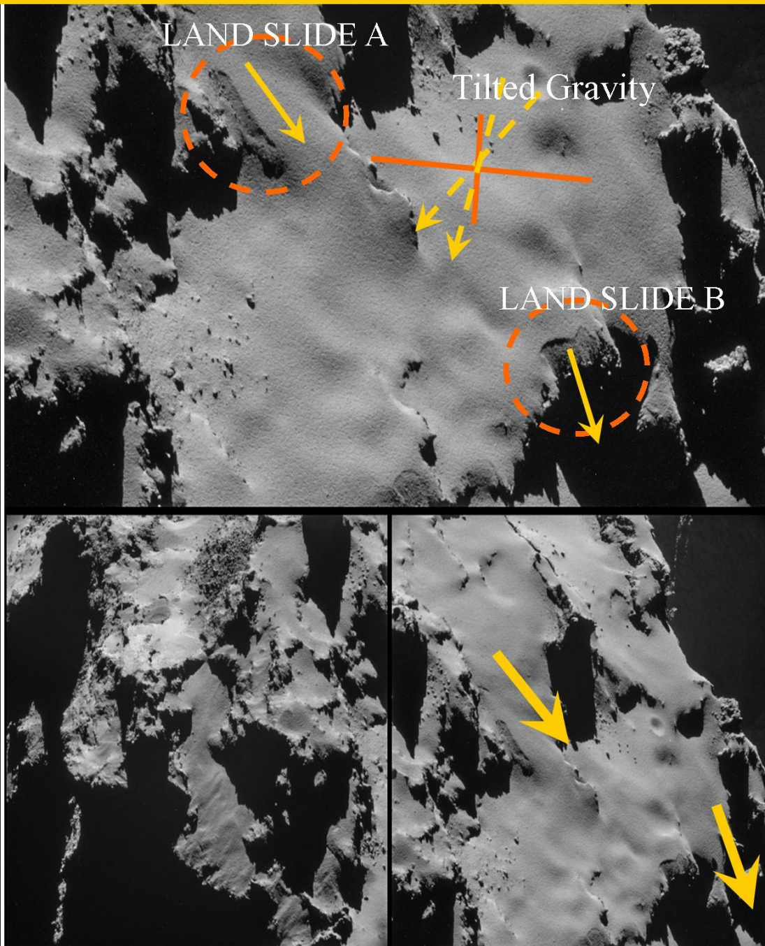
Figure34, Anomalous non perpendicular surface Gravity problem.
