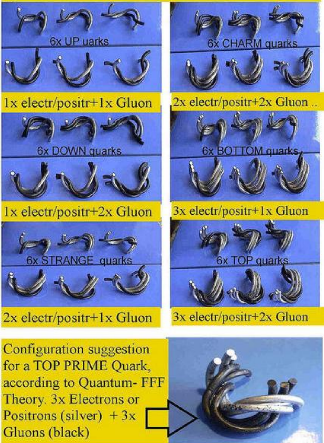
Figure 21, 5x different shaped Photon/Gluons can combine with the two propeller shapes of the Electron and Positron to form all coloured (QCD) Quarks and even a so called Top Prime Quark. The Muon and Tau particle are supposed to be the same as the Down quark, respectively the Charm quark.
