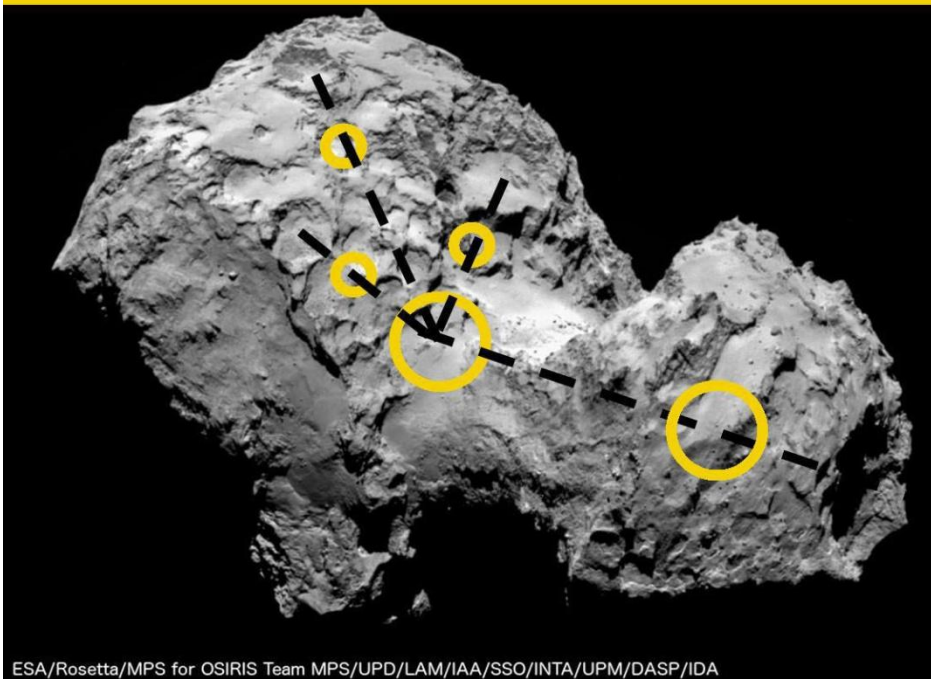
Figure: 26, Proposal for the origin of circular craters at Comet 67p C-G.
