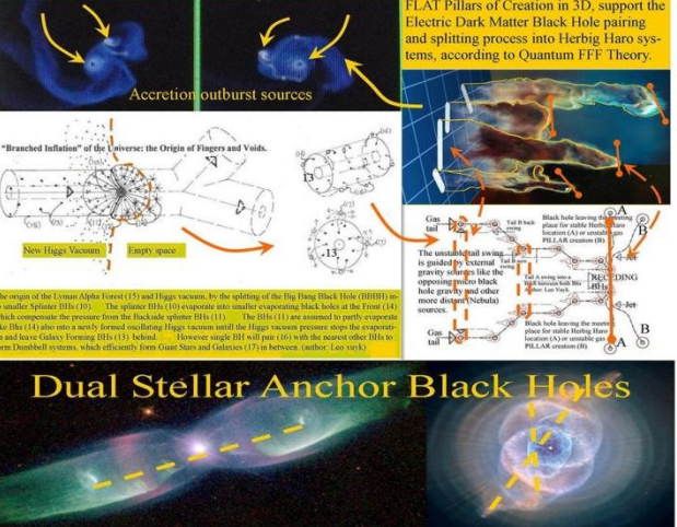
Figure: 19, The great misconception in astronomy and astrophysics.
