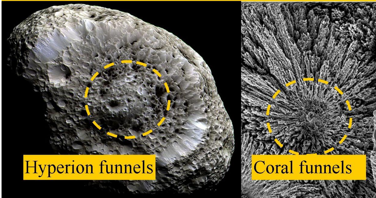
Figure , 31. Cracks in the Carbon dust layer.
