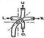
(Above) Alternative Feynman diagrams for electron-positron attraction and electron-electron repulsion by Dipole Repeller system.
