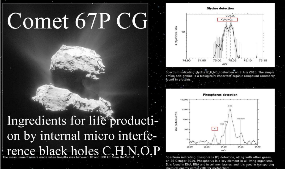
Fig 5. Ingredients for life production by internal micro interference black hole quantum knots.
