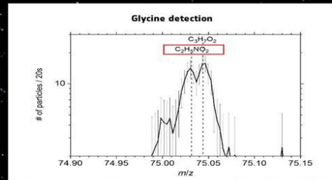
Spectrum indicating glycine [C 2 H 5 NO 2 ] detection on 9 July 2015. The simple amino acid glycine is a biologically important organic compound commonly found in proteins.
