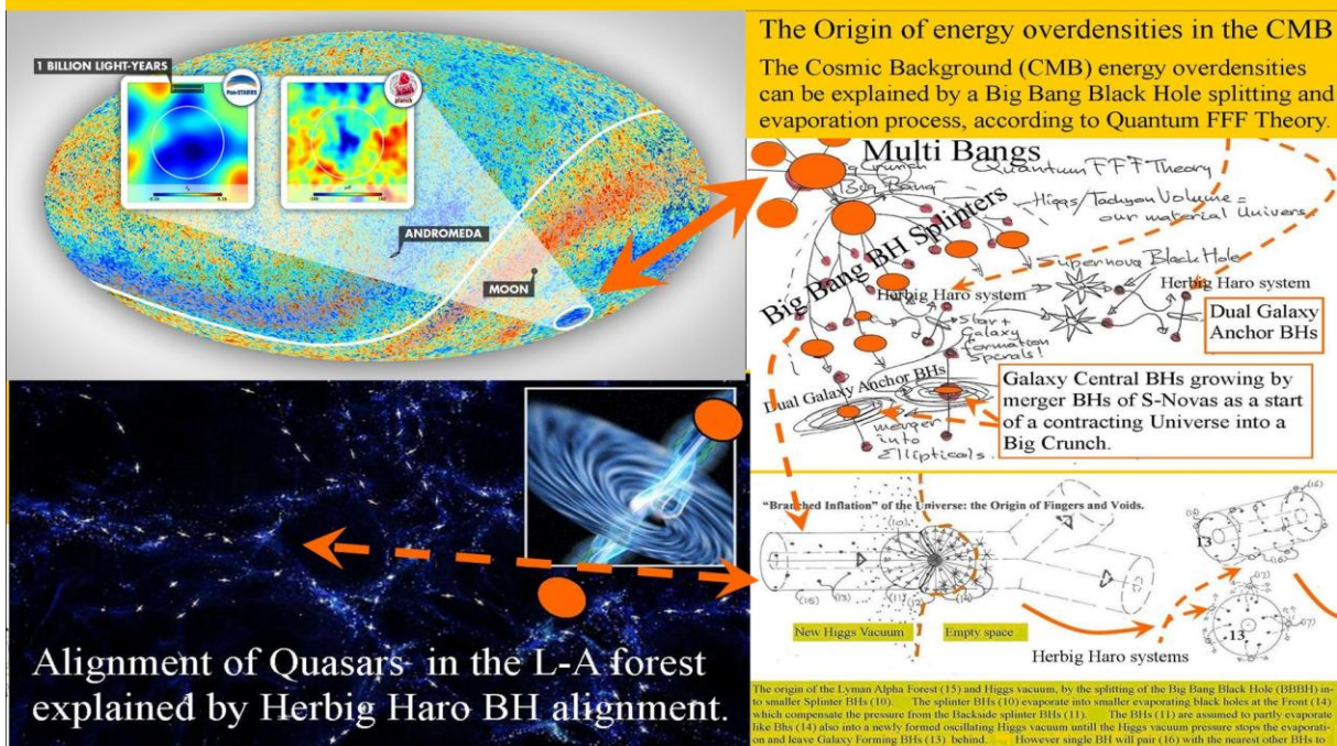
Figure: 35. Alignment of Supervoid and Cold spot including Quasars support the idea of branched inflation by Big Bang Black Hole nucleus splitting and evaporation process .
