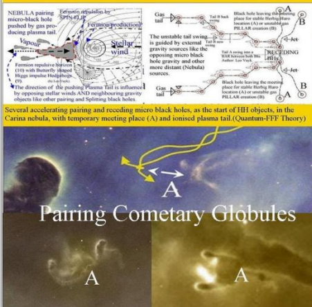
Figure: 19, The great misconception in astronomy and astrophysics.
