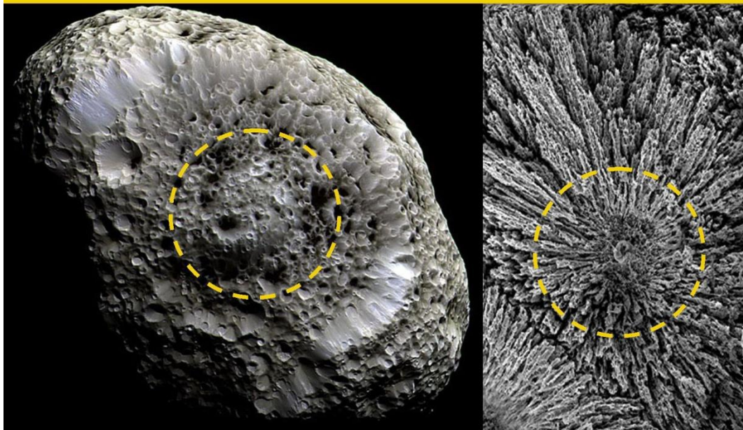
Figure 28, Hyperion , a former Comet.
