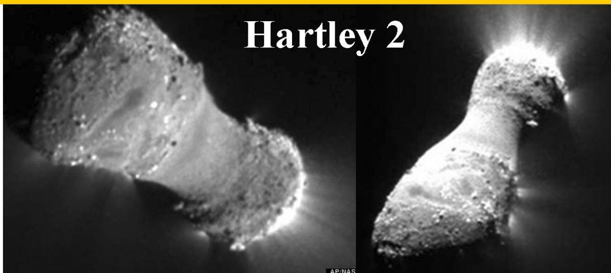
Figure: 23, both comets more in detail.
