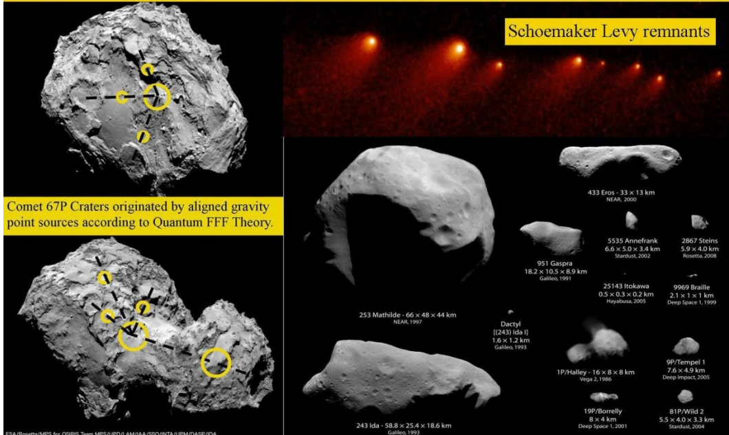
Figure 27, What can we learn about multiple nuclear comets?
