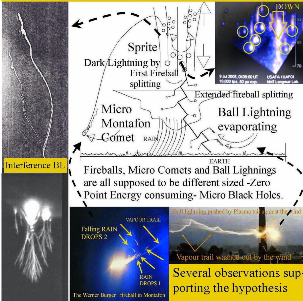
Figure: 1, Creation of Interference black holes and its plasma production ( vapour trail of ball lightning Sprites Micro Comets and Fireballs. )
