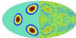
Figure 3, Wavefunction collapse in the Charge Parity ( Time) symmetric Raspberry multiverse.
