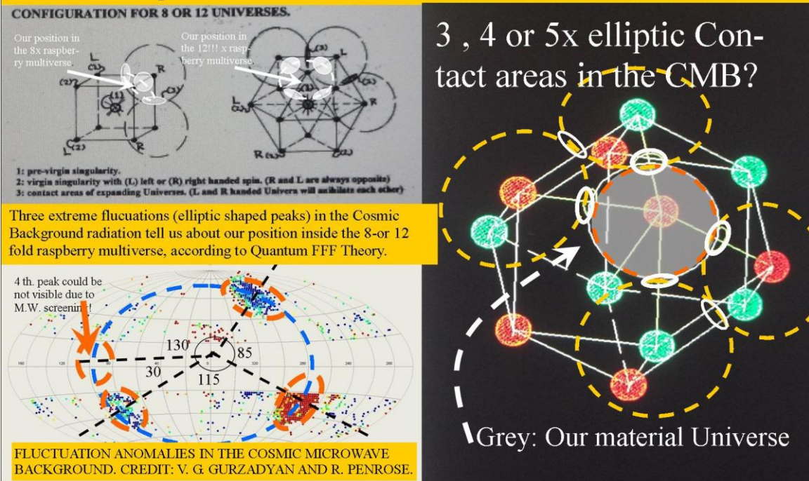
Figure 5, The number of elliptic Fluctuation Anomalies in the CMB suggested by Gurzadyan and Penrose.
