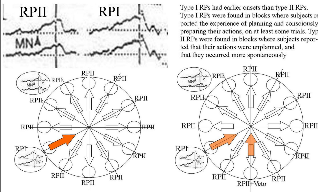
Figure 6, Preplanning (RPI) and (instant Veto/or acceptance) reaction (RPII) represented for a 12 fold multiverse.
