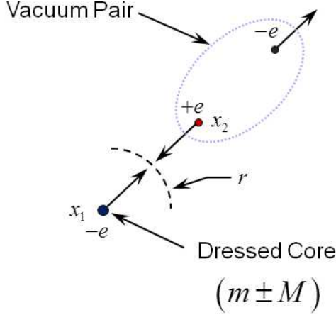
FIG. 2: Dressed core electron interacts with opposing vacuum current resulting in an exchange of the core and vacuum electrons and a sign reversal of the EDC scattering amplitude relative to the core.
