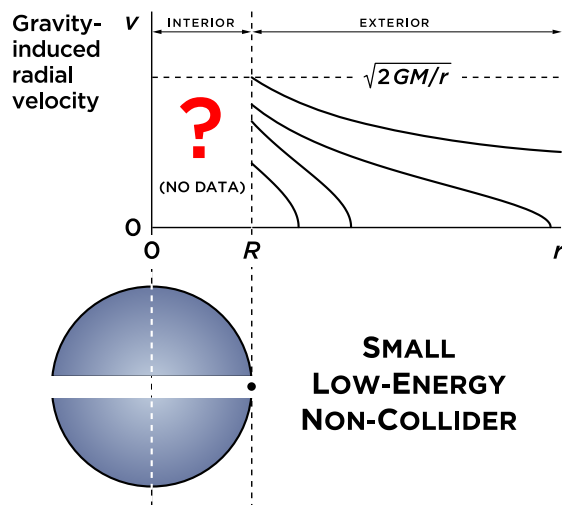
Fig. 2 Huge gap in gravitational data. Rotonians strongly urge filling it.
