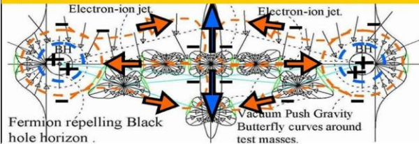
Figure 19, Binary star production .
