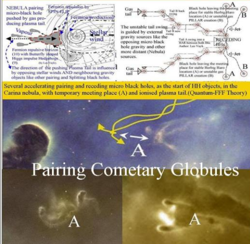
Figure: 34, the great misconception in astronomy. Pairing Cometary globules are: small solar mass black holes seem able to combine into Herbig Haro systems to form Bok globules with failed stars in between.
