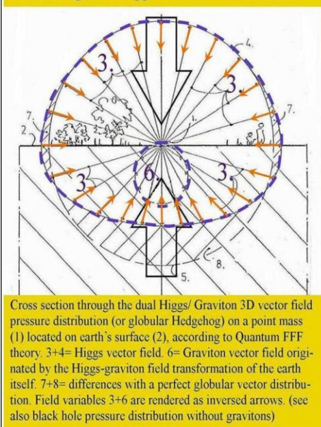
Figure 20, equivalence between gravity and acceleration does not hold in Q-FFF theory.
