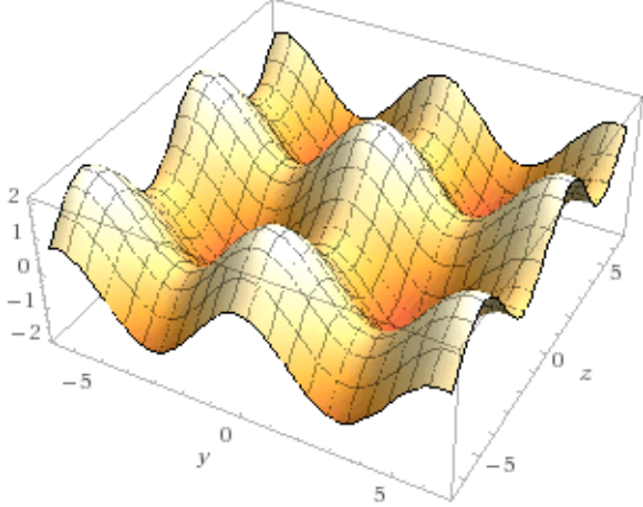
Figure 5. Finding the global maximum.
