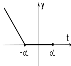
Graph of the trajectory y = r_\alpha(t) for \alpha \in (0, \infty) .
