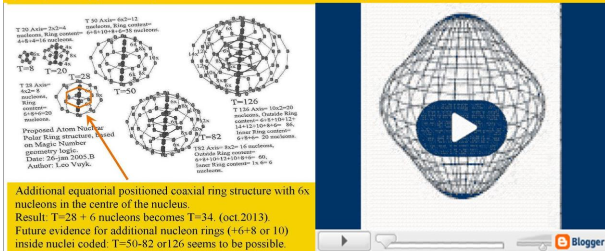
Figure: 3, Axial Ring structure of Atomic Nuclei according to Quantum FFF Theory.
