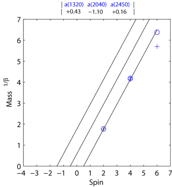
FIGURE 20. Positive parity a_1
