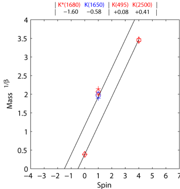
FIGURE 28. Positive and negative parity K2
