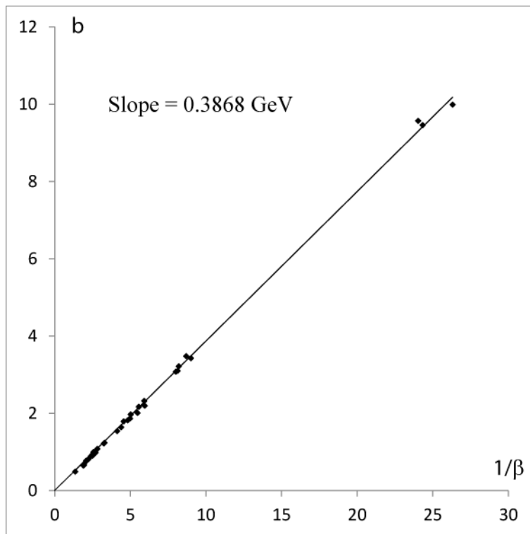
FIGURE 48. b as a function of 1/\beta
