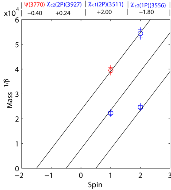
FIGURE 41. Positive and negative parity \chi_{c1} and \psi_{c1}
