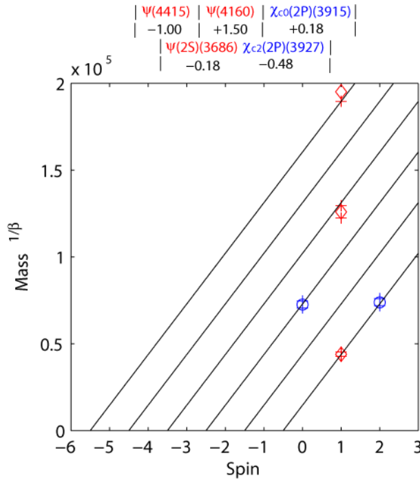
FIGURE 43. Positive and negative parity \chi_{c3} and \psi_{c3}
