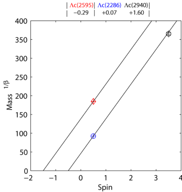
FIGURE 29. Positive and negative parity \Lambda_c 1
