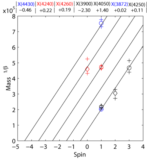
FIGURE 39. Positive and negative parity X1
