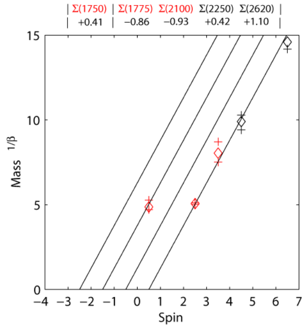
FIGURE 13. Negative parity \Sigma 1
