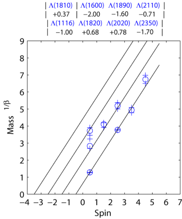
FIGURE 9. Positive parity \Lambda 1
