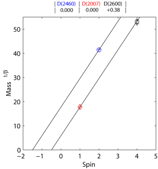
FIGURE 35. Positive and negative parity D2
