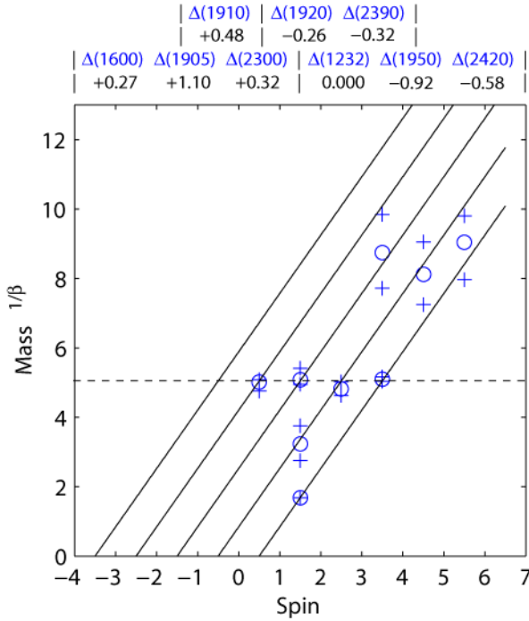
FIGURE 7. Positive parity \Delta 1
