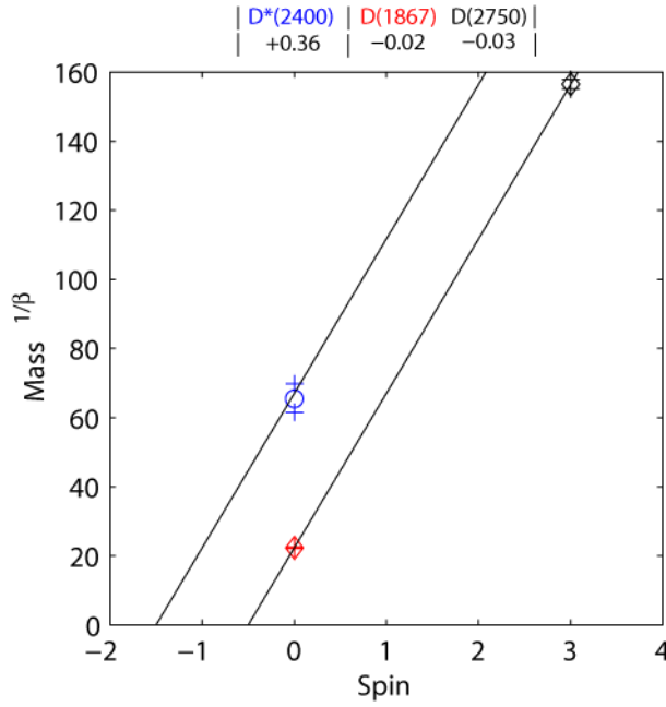
FIGURE 34. Positive and negative parity D1
