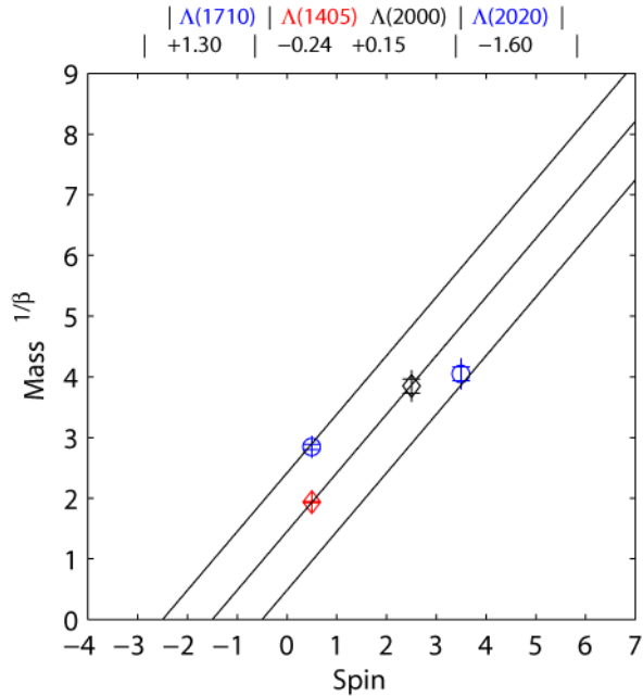
FIGURE 11. Positive and negative parity \Lambda_2
