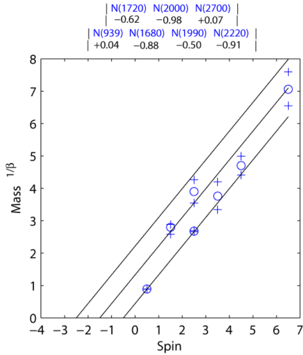
FIGURE 3. Positive parity N1
