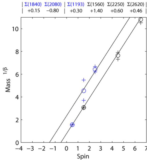
FIGURE 16. Positive parity \Sigma 3
