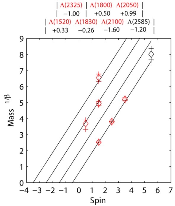
FIGURE 10. Negative parity \Lambda 1
