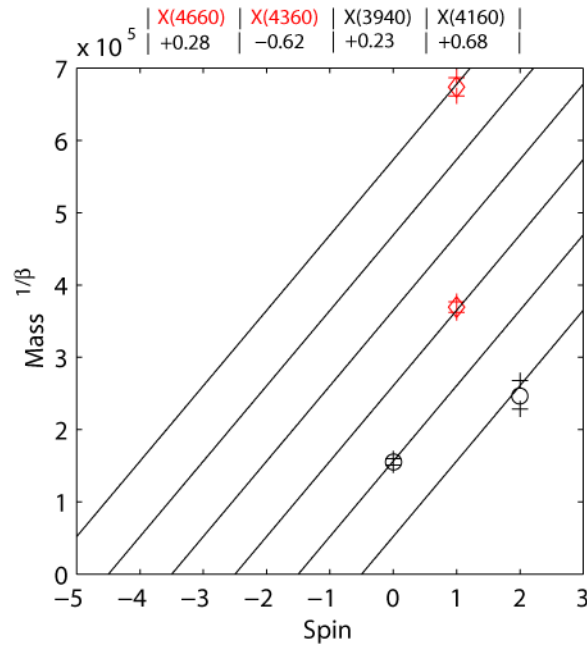
FIGURE 40. Positive and negative parity X2
