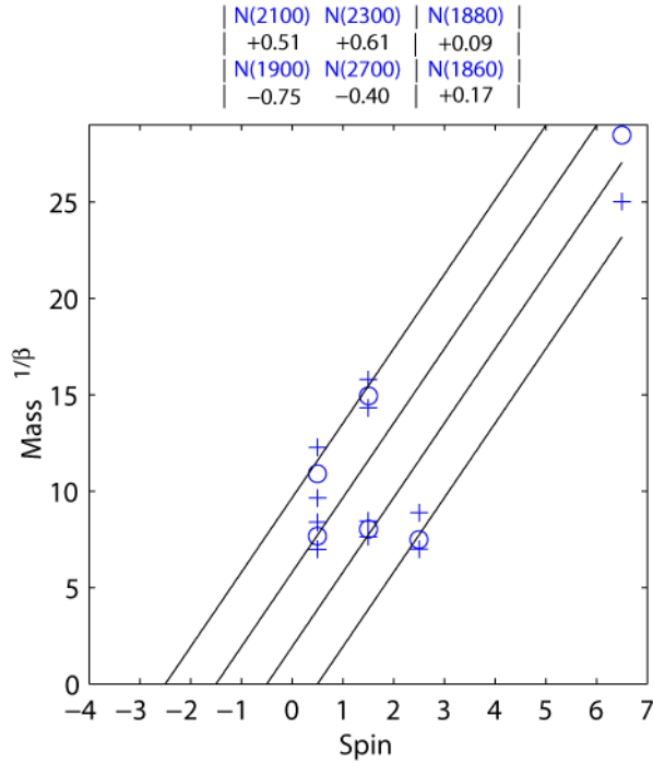
FIGURE 5. Positive parity N2
