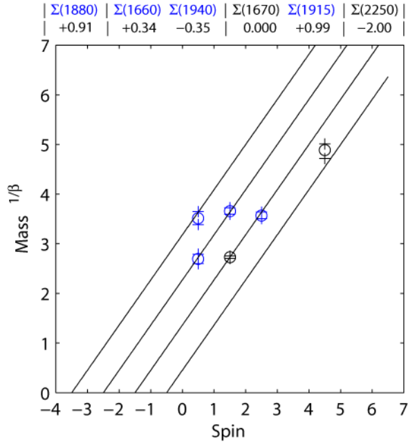
FIGURE 14. Positive parity \Sigma 2
