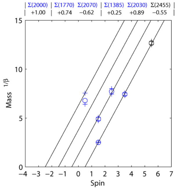
FIGURE 12. Positive parity \Sigma 1
