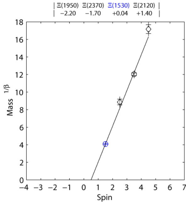
FIGURE 19. Positive and negative parity \Xi 2
