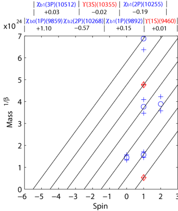
FIGURE 44. Positive and negative parity \chi_{b1} and Y1
