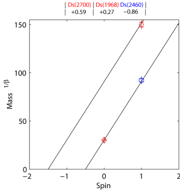
FIGURE 36. Positive and negative parity Ds1
