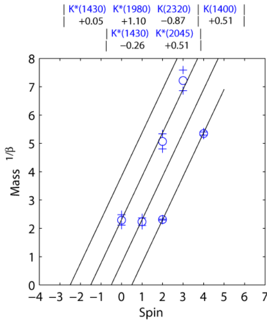
FIGURE 26. Positive parity K1
