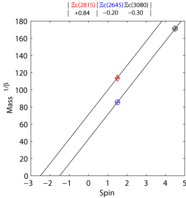
FIGURE 33. Positive and negative parity \Xi_c2
