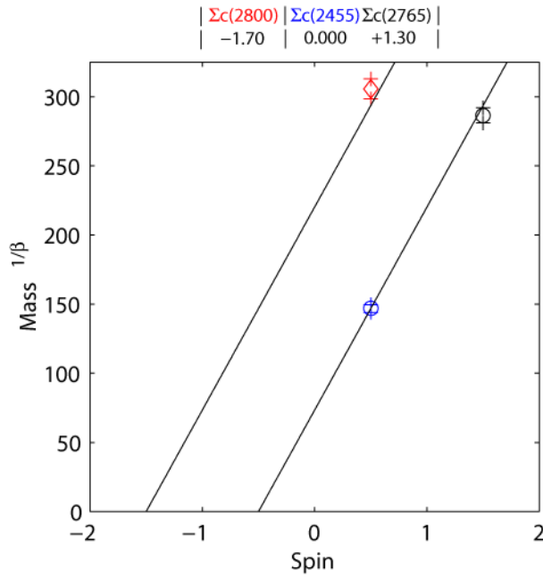
FIGURE 31. Positive and negative parity \Sigma_c 1
