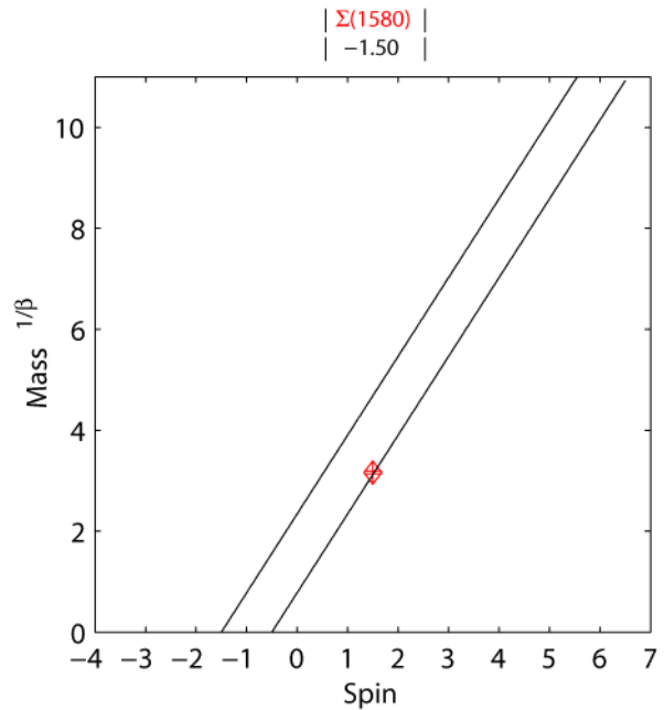
FIGURE 17. Negative parity \Sigma 3
