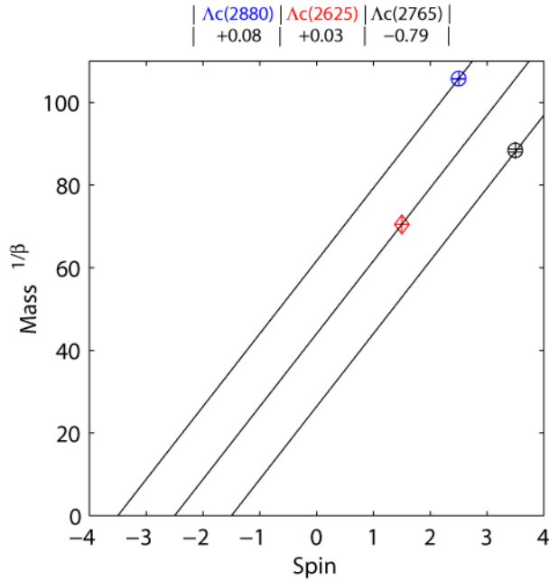
FIGURE 30. Positive and negative parity \Lambda_c2
