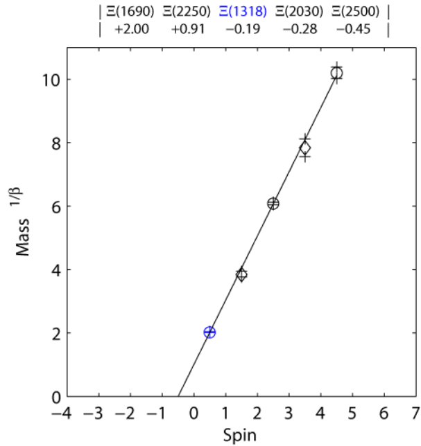
FIGURE 18. Positive and negative parity \Xi 1
