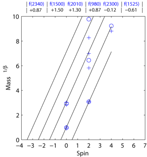
FIGURE 25. Positive and negative parity f_2 and \omega_2
