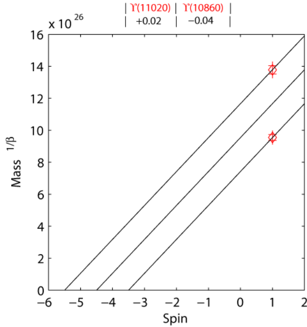
FIGURE 46. Straight lines \chi_{b3} and Y_3
