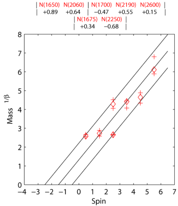
FIGURE 4. Negative parity N1
