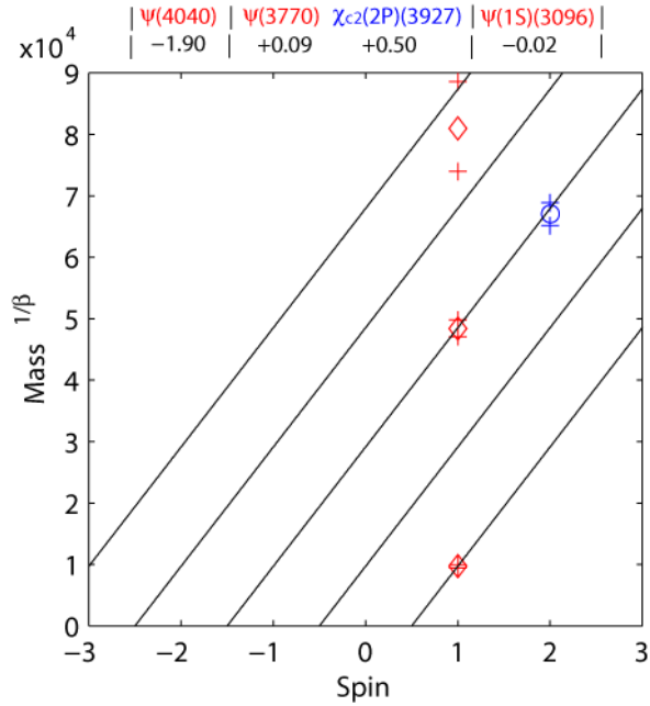
FIGURE 42. Positive and negative parity \chi_{c2} and \psi_{c2}
