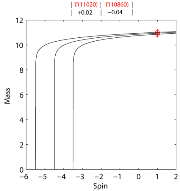
FIGURE 47. Curved lines \chi_{b3} and Y_3
