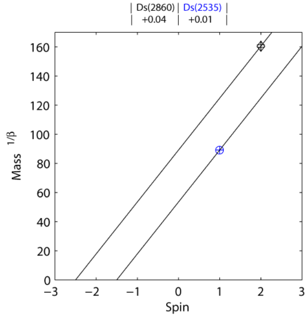
FIGURE 38. Positive and negative parity Ds3
