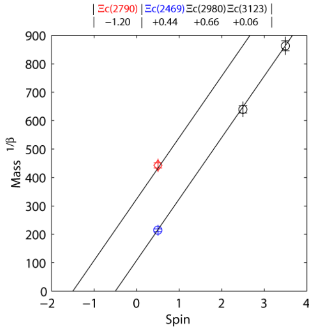
FIGURE 32. Positive and negative parity \Xi_c 1
