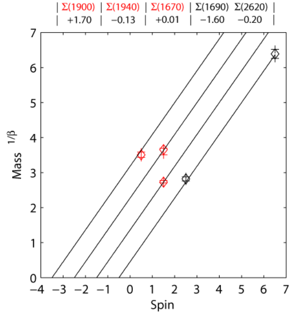
FIGURE 15. Negative parity \Sigma 2
