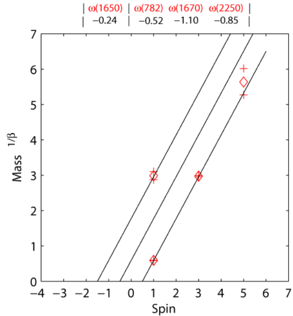
FIGURE 24. Negative parity ω1
