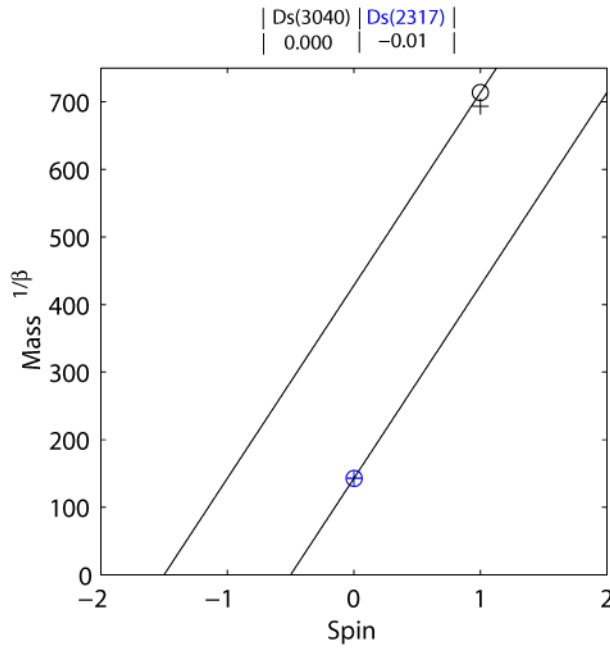
FIGURE 37. Positive and negative parity Ds2
