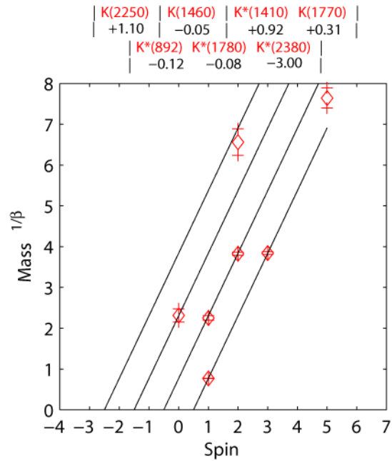
FIGURE 27. Negative parity K1
