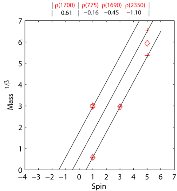
FIGURE 21. Negative parity \rho_1
