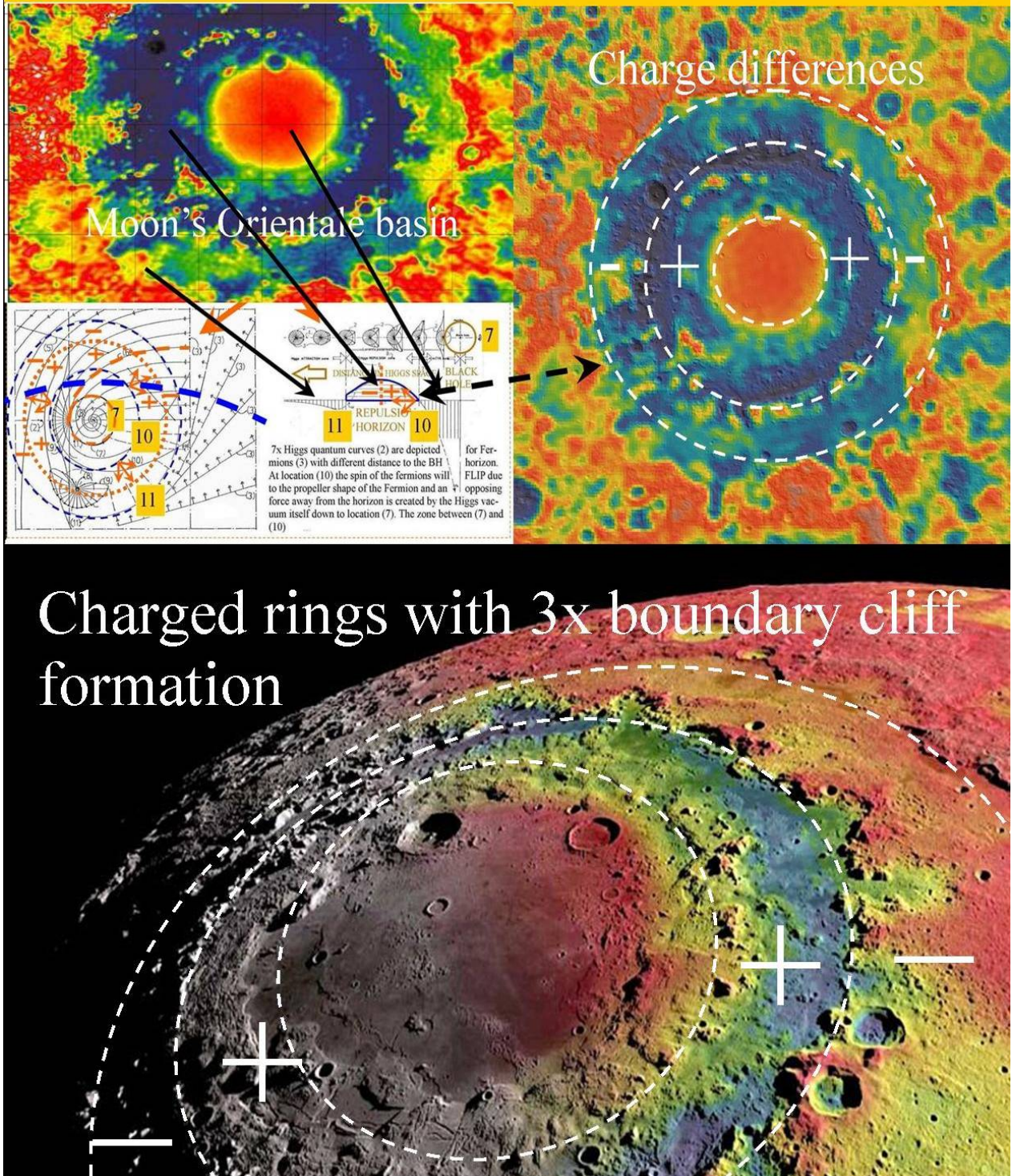
Figure 1, The cliff formation by electrostatic horizontal pressure and extra gravity.
