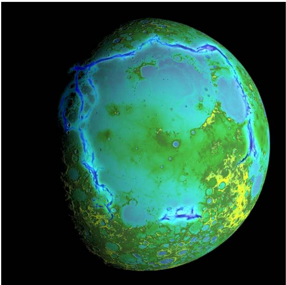
Figure 0, Recent observations show that even the moon seems to grow if we look at the the rifts of Oceanus Procellarum.
