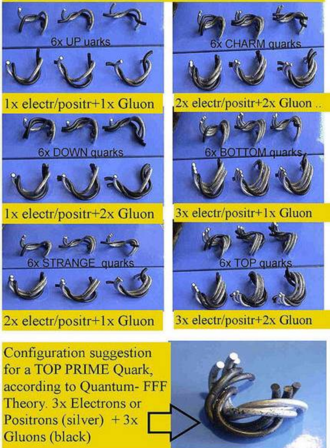
Figure 14, 5x different shaped Photon/Gluons can combine with the two propeller shapes of the Electron and Positron to form all coloured (QCD) Quarks and even a so called Top Prime Quark. The Muon and Tau particle are supposed to be the same as the Down quark, respectively the Charm quark.
