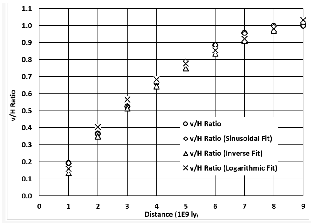
FIGURE 4. v/H Ratio vs. Distance
