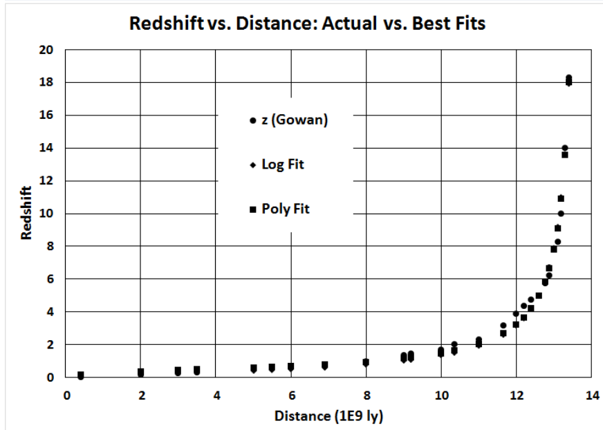
FIGURE 2. Redshift vs. Distance
