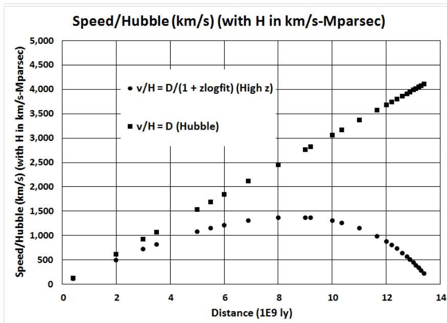
FIGURE 3. Recession Speed (Scaled to Hubble Constant) vs. Distance
