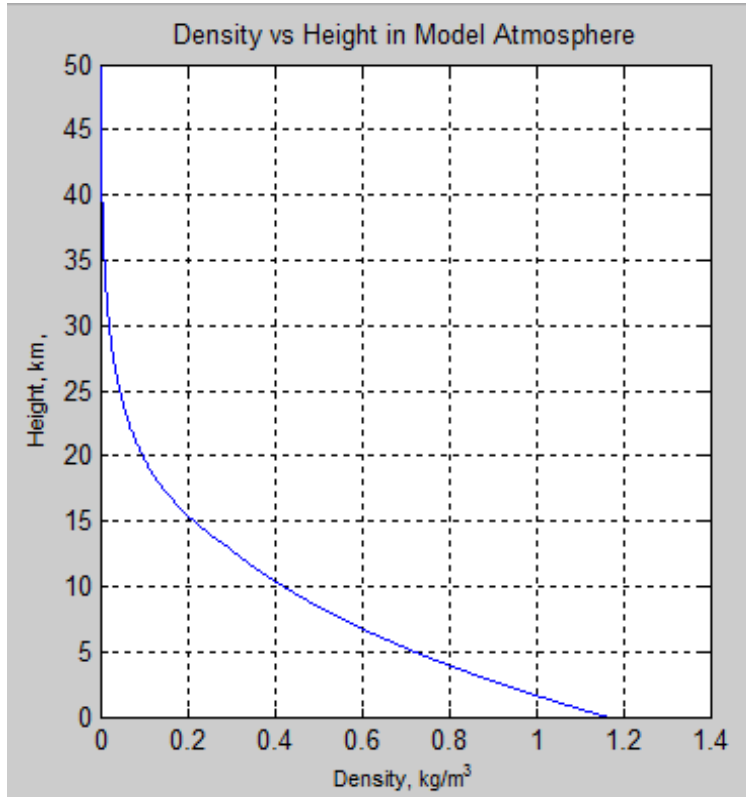
FIGURE 1. Atmospheric Density vs. Altitude
