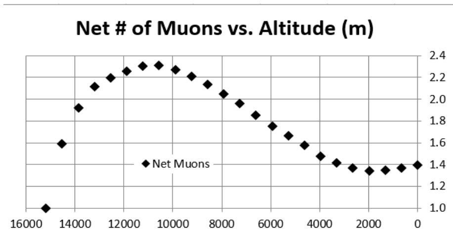
FIGURE 3. Net Number of Muons vs. Altitude (m)
