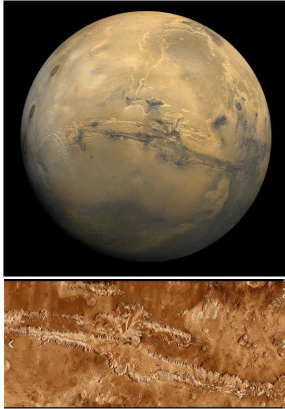
Figure 1. Valles Marineris [3]
