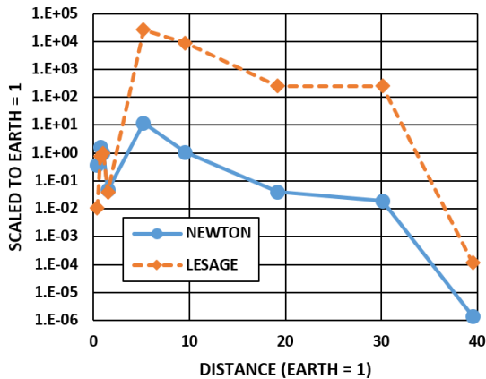
FIGURE 3. Newtonian vs. LeSagian Gravitational Force vs. Distance for the Nine Planets
