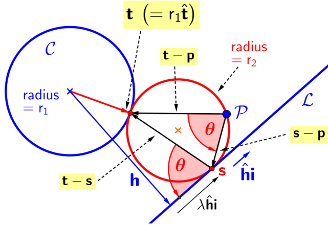
Figure 3.4: A pair of equal angles that might provide a basis for solving the problem via rotations.)
