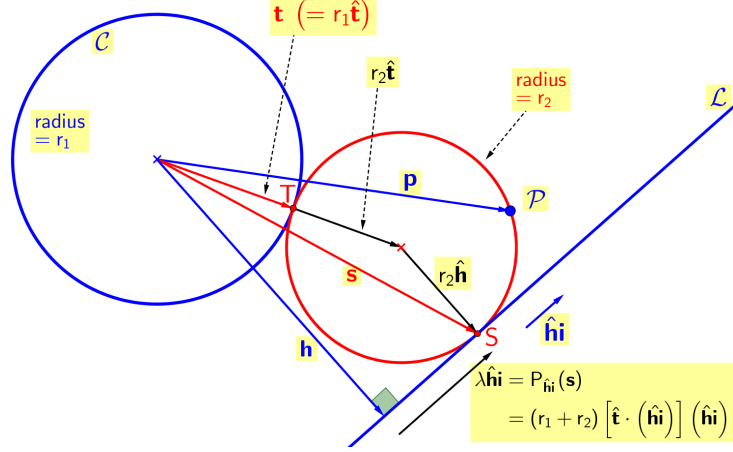
Figure 3.3: Further steps in choosing elements for capturing the geometric content of the problem. (See text for explanation.)
