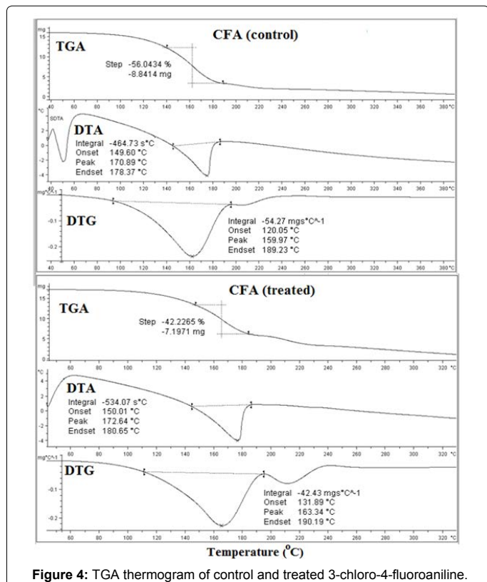
Figure 4: TGA thermogram of control and treated 3-chloro-4-fluoroaniline.
