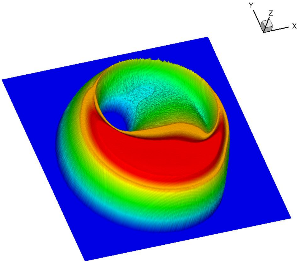
Figure 5 – Same of Figure 4 but here rotated around the z-axis of 240^\circ to see the black-hole surroundings from another viewpoint.
