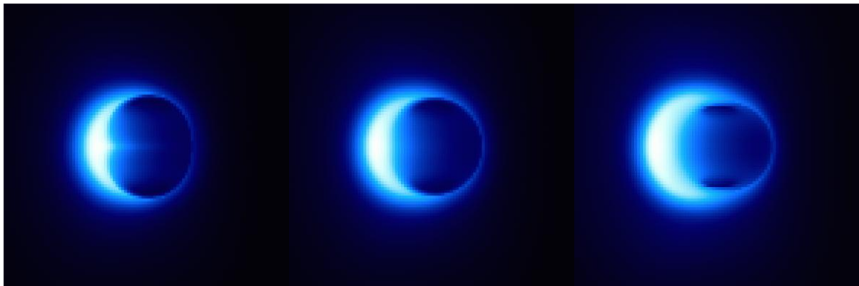
Figure 1 – Possible shadow shapes in the neighborhood of a black hole (D. Psaltis and A. Broderick, 2016).
