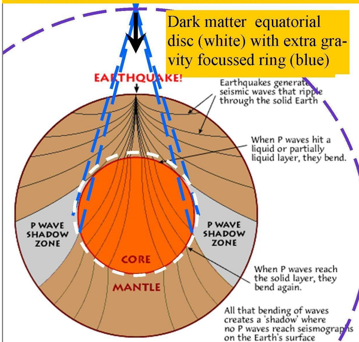
Figure 12, Flyby anomaly explained by earth internal rings of cometary dark matter black hole nuclei.
