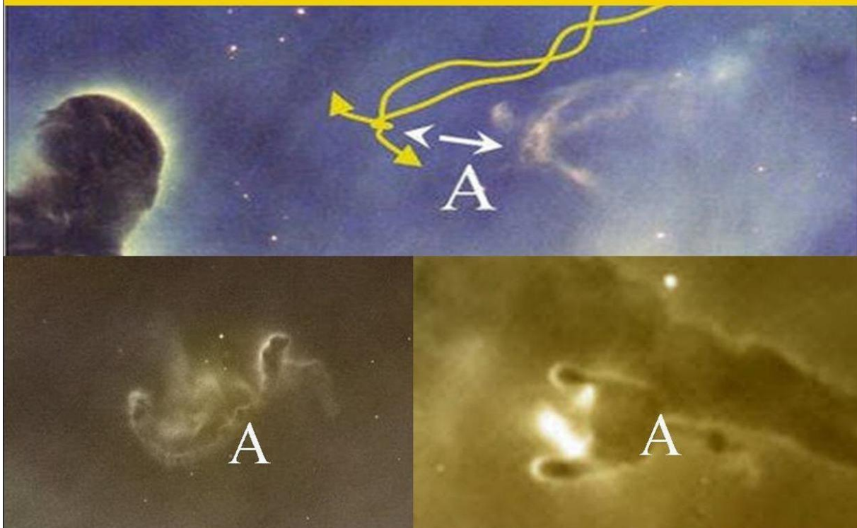
Figure 20, Splitting and pairing electric dark matter blackholes.
