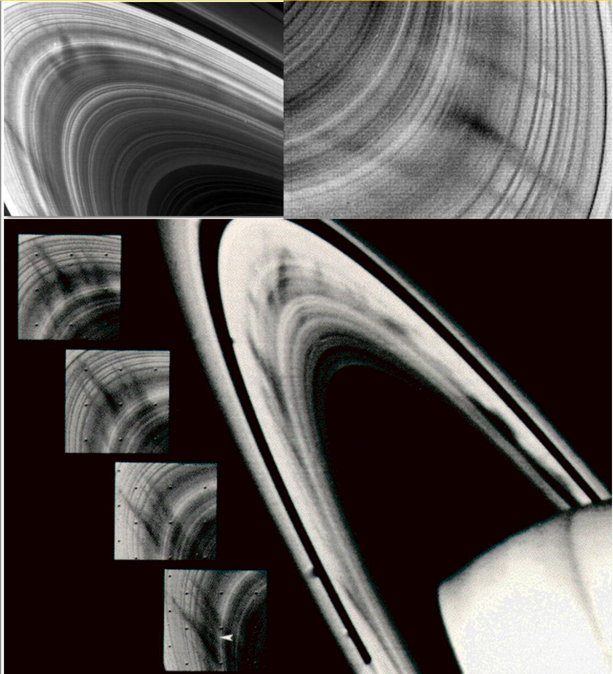
Figure 15, Temporary spokes inside Saturn's ring, by the pencil shaped gravity influence of aligned internal dark matter black holes. ( former crashed Comet nuclei)
