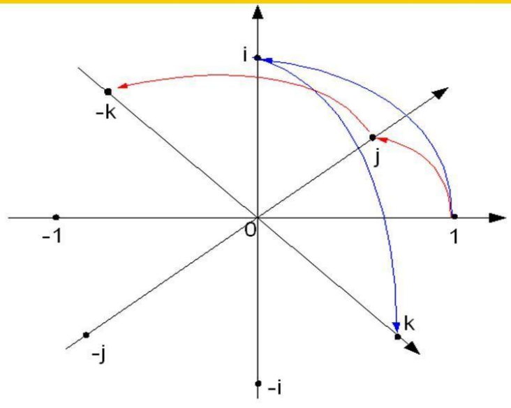
Figure 22, 4D Quaternion rotations compared with Quantum FFF 90 degr. hinging models.
