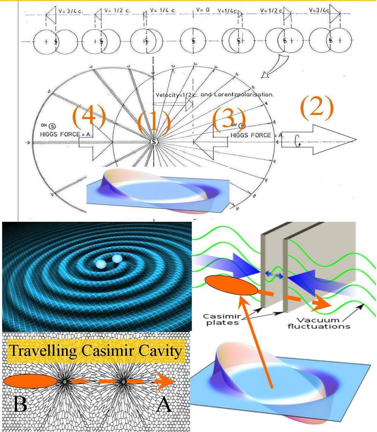
Figure 21, LIGO gravity lawn sprinkler effect.
