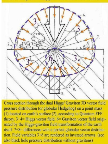
Figure 17, Quantum gravity.
