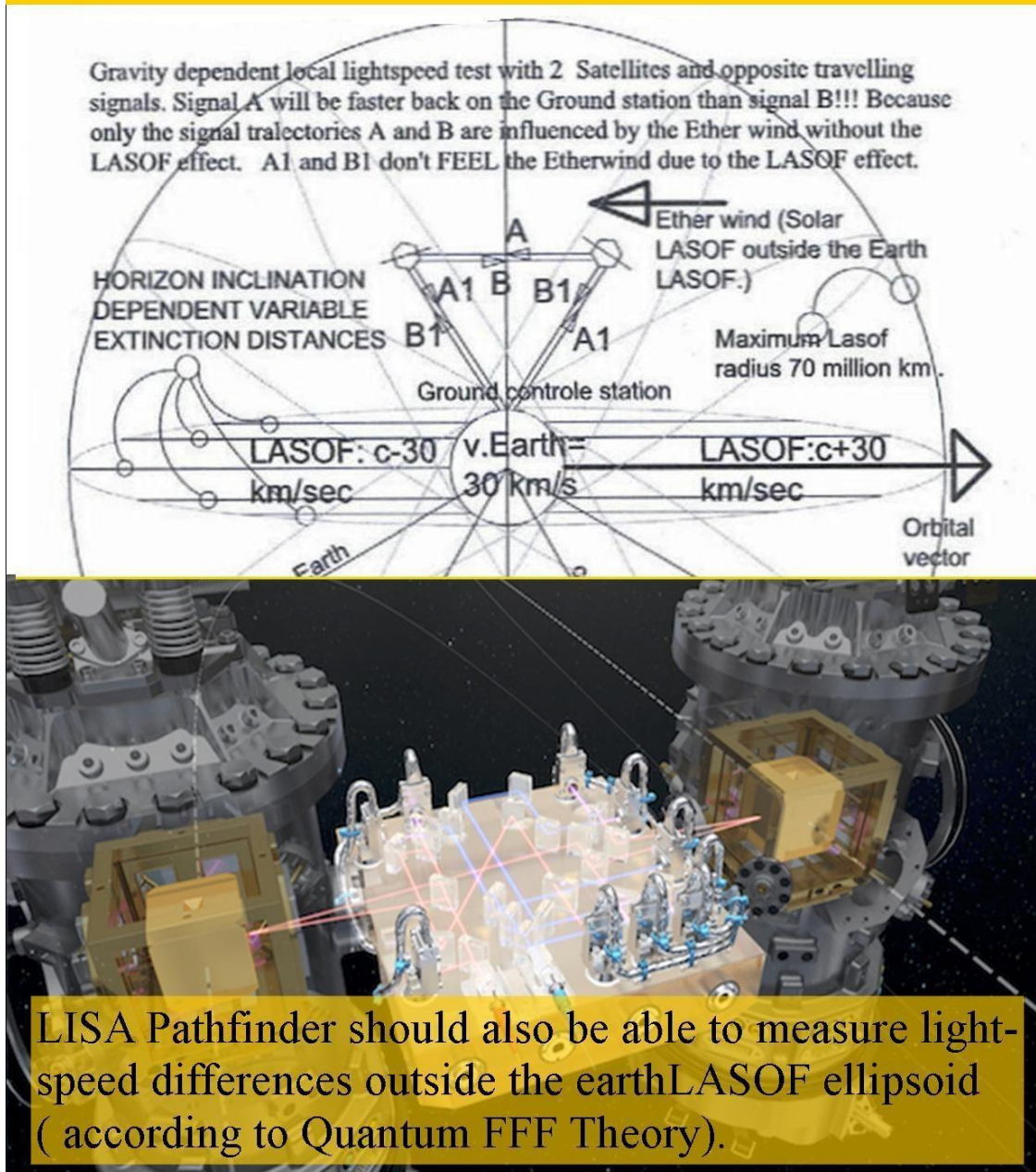
Figure 10, Gravity dependent lightspeed anomalies.
