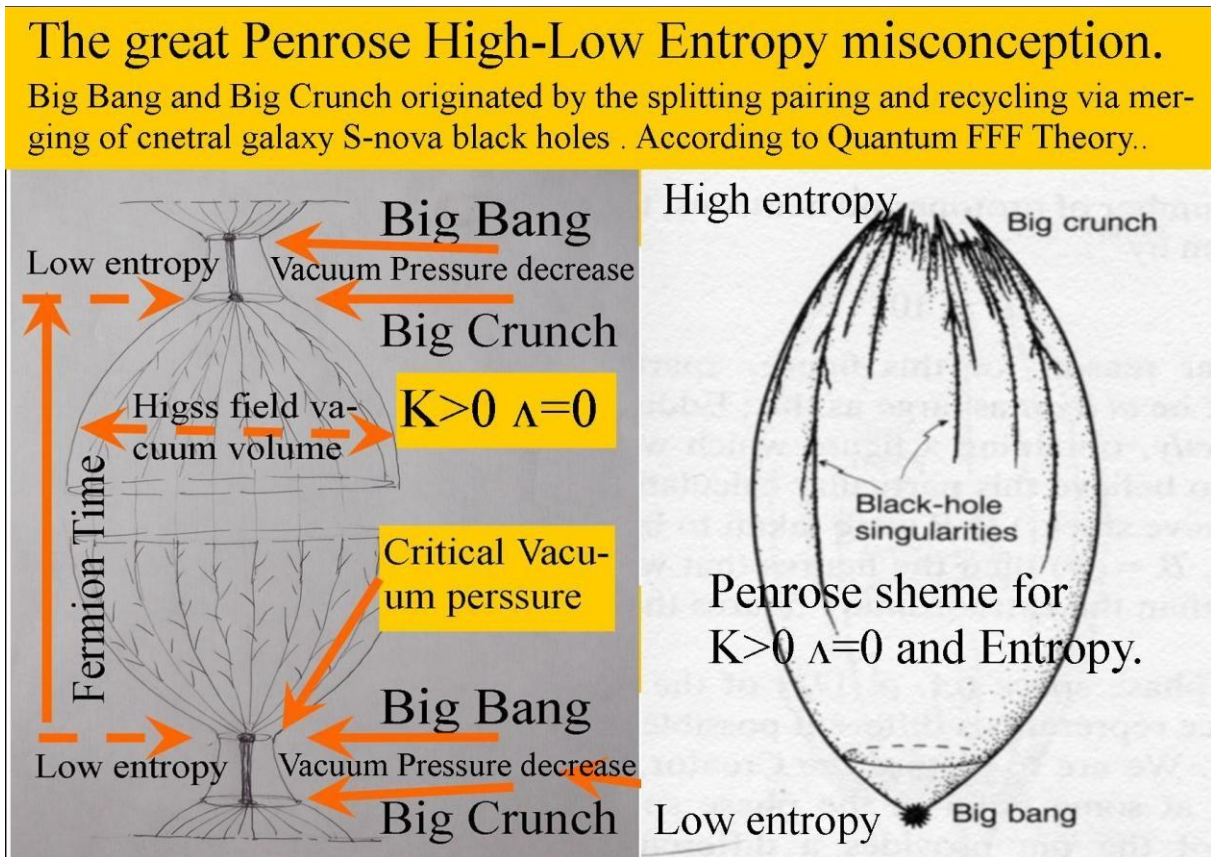
Figure 11, The cyclic Universe with Entropy development in contrast with Penrose.
