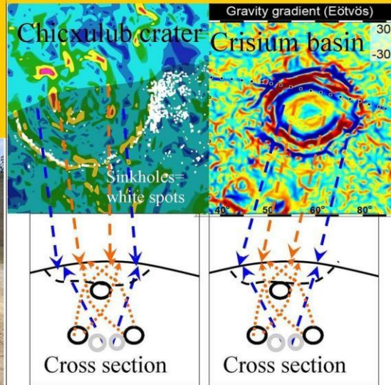
Figure 16, Anomalous gravity effects on Earth and Moon also by aligned internal dark matter black holes ( former Comet nuclei)
