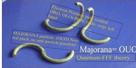
Figure 7, particle schemes of Quantum FFF Theory.
