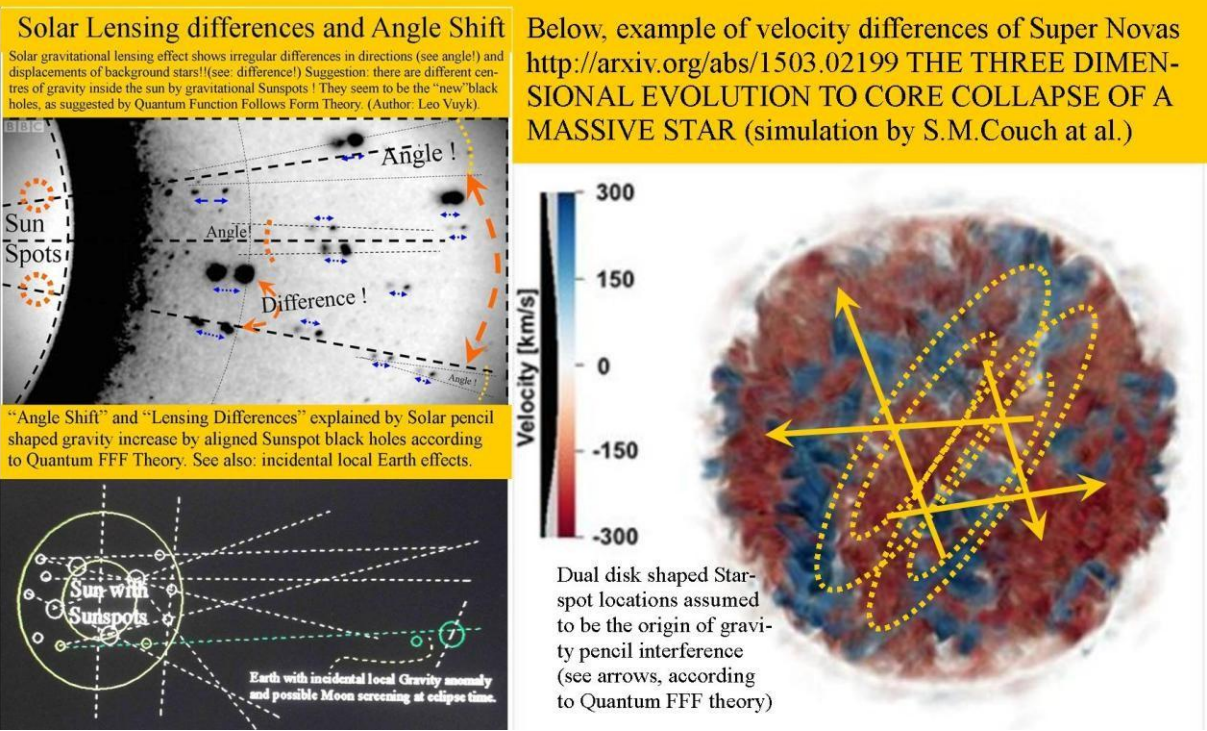
Figure 13, Sunspot dark matter black hole effect on background stellar lensing directions.
