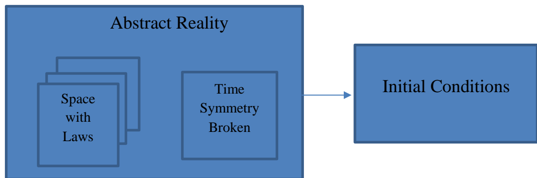
Figure Four. Hypothetical Framework for Spacetime
