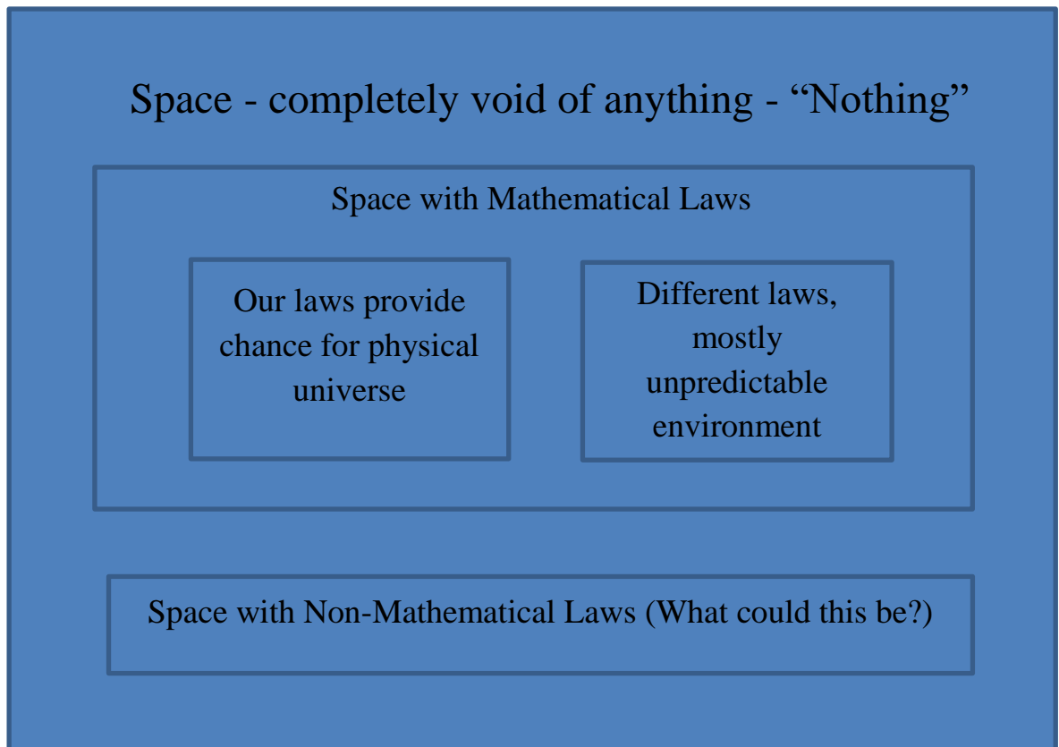
Figure Three. Space and Nothing
