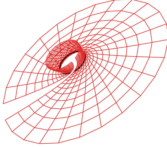
Fig.3 P_2(s;t) as a member of the surface family and its common natural geodesic lift \bar{\alpha}
