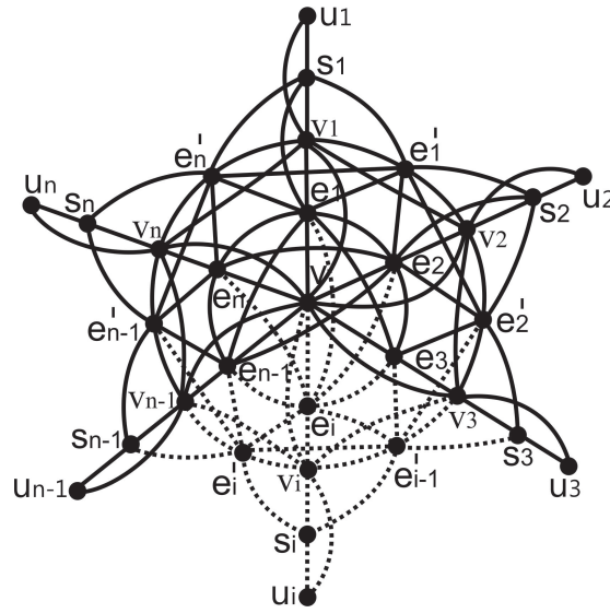
Fig.6 Total Graph of Helm Graph T(H_n) .
