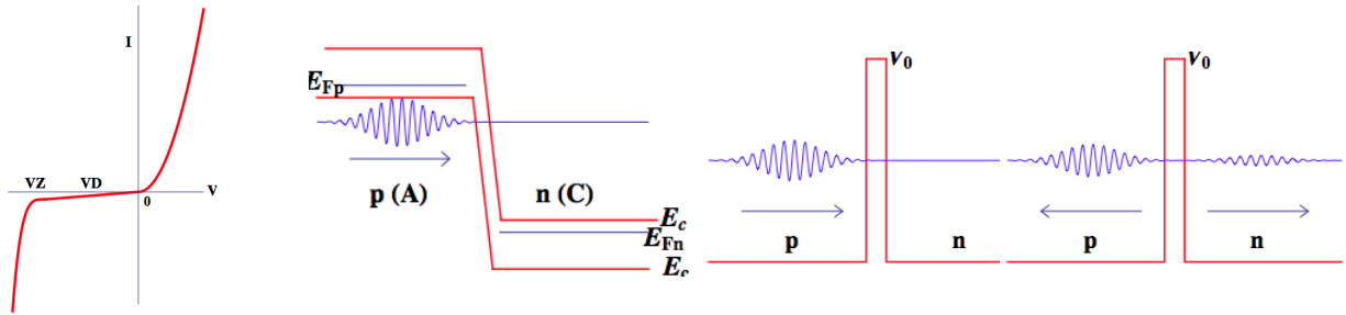
Figure 8: Left: Current-Voltage (IV) characteristics for a Zener Diode. VZ = -3.3V is the Zener voltage, and VD \approx -1.5V is the operating voltage for the diode in Fig.9. V > 0 is the forward bias region, and V < 0 is the reverse-bias region. The current near VD is very small and occurs only because of wave function quantum tunnelling through the potential barrier, as shown to the Right: Electron before tunnelling, in reverse-biased Zener diode, from valence band in doped p semiconductor, with hole states available, to conduction band of doped n semiconductor. A and C refer to anode and cathode labelling in Fig.9. E_c is bottom of conduction bands, and E_v is top of valence bands. E_{Fp} and E_{Fn} are Fermi levels. There are no states available in the depletion region. Next: Schematic for electron wave packet incident on idealised effective interband barrier in a pn junction, with electrons tunnelling A to C , appropriate to reverse-bias operation. Next: Reflected and transmitted wave packets after interaction with barrier. Energy of wave packet is less than potential barrier height V_0 . The wave function transmission fluctuations and collapse to one side or the other after barrier tunnelling is now experimentally demonstrated to be caused by passing space fluctuations.
