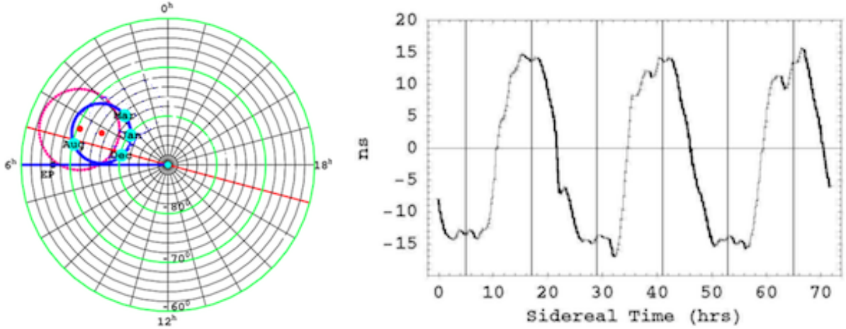
Figure 3: Left: South celestial pole region. The dot at RA=4.3^h , Dec=75^\circ S , and with speed 486\text{km/s} , is the year-averaged direction of motion of the solar system through space determined from NASA spacecraft Earth-flyby Doppler shifts [64], as revealed by the EM radiation speed anisotropy. The thick circle centred on this direction is the observed velocity direction for different months of the year, caused by Earth orbital motion and Sun 3-space inflow. The corresponding results from the 1925/26 Miller gas-mode interferometer are shown by 2nd dot and its aberration circle. For December 8, 1992, the speed is 491\text{km/s} from direction RA=5.2^h , Dec=80^\circ S , see Table 2 of Cahill [64]. EP is the pole direction of the plane of the ecliptic, and so the space flow is close to being perpendicular to the plane of the ecliptic. Right: Variations in travel time from DeWitte's RF coaxial cable experiment of 1991, resulting in a speed of 500\text{km/s} with RA=5\text{hrs} .
