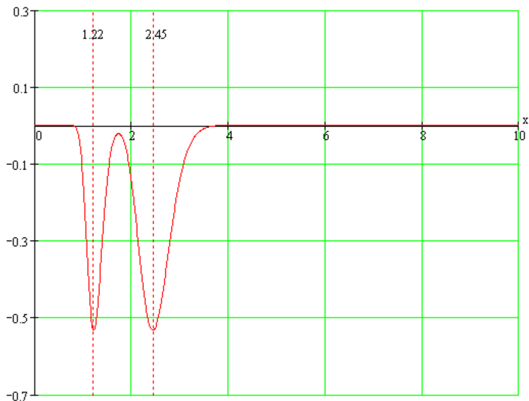
Figure OP3. Function PES - Field potential - changes of the structural component of fundamental matter field
