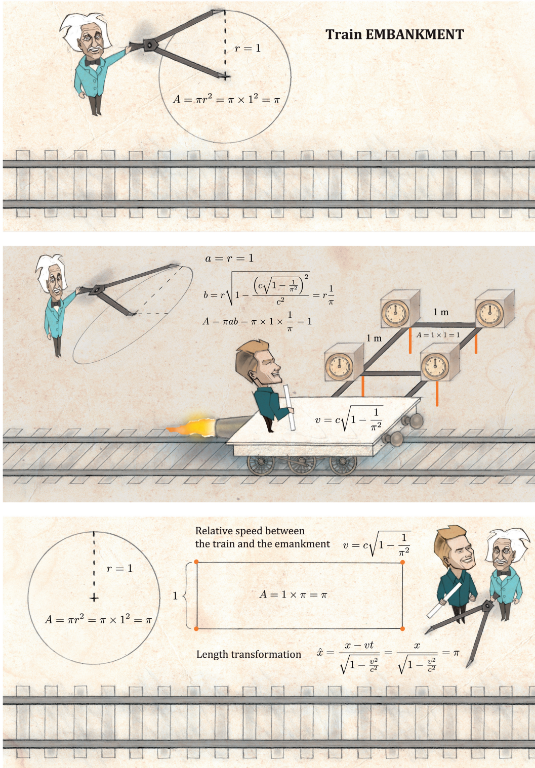
Figure 1: Squaring the Circle.
