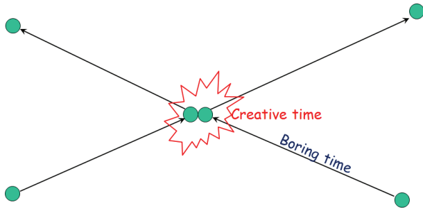
FIG. 2: Sketch of two colliding classical particles. Initially they merely move along straight lines, nothing happens. Next, they collide, the very detail of this process depends on infinitesimal digits of the initial conditions and of their shapes. Finally, the two particles continue again along boring straight lines.
