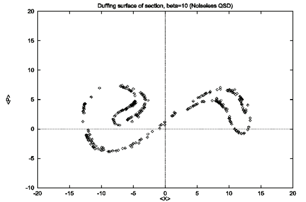
FIG. 4: Poincaré section of the forced and damped quantum Duffing oscillator in the chaotic regime, described by the Quantum State Diffusion model of open quantum systems [14]. Note that the axes represent quantum expectation values of position and momentum. This strange attractor is essentially identical to its classical analog.
