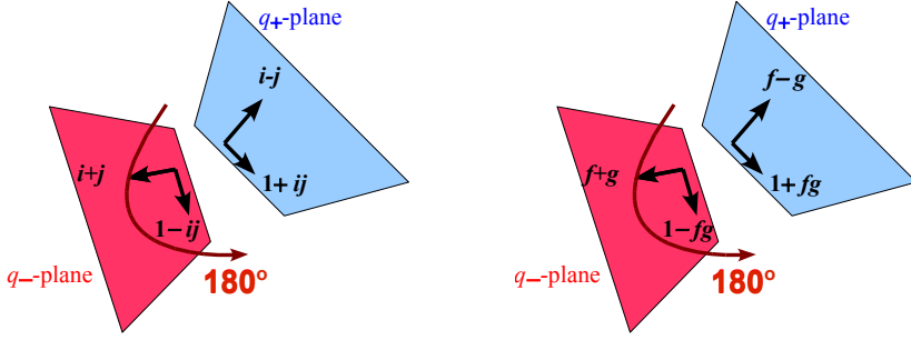
FIGURE 1. Geometric pictures of the involutions i(.)j and f(.)g as half turns.
