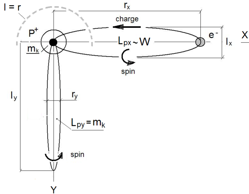
Fig.1: Scheme of a neutrino formation
