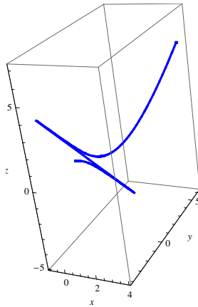
Figure 1: The spacelike general helix \alpha in G_3^1 with \kappa_\alpha = \frac{1}{u} and \tau_\alpha = \frac{-2}{u} .
