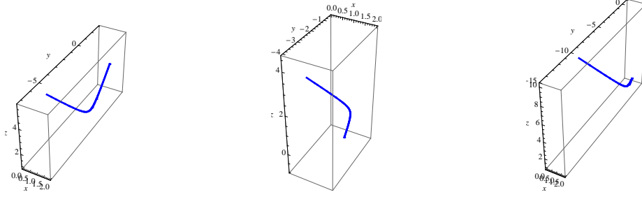
Figure 2: The \mathbf{e}_1\mathbf{e}_2 , \mathbf{e}_1\mathbf{e}_3 and \mathbf{e}_1\mathbf{e}_2\mathbf{e}_3 Smarandache curves of \alpha .
