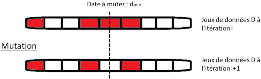
figure III.3 : Illustration du principe de mutation
