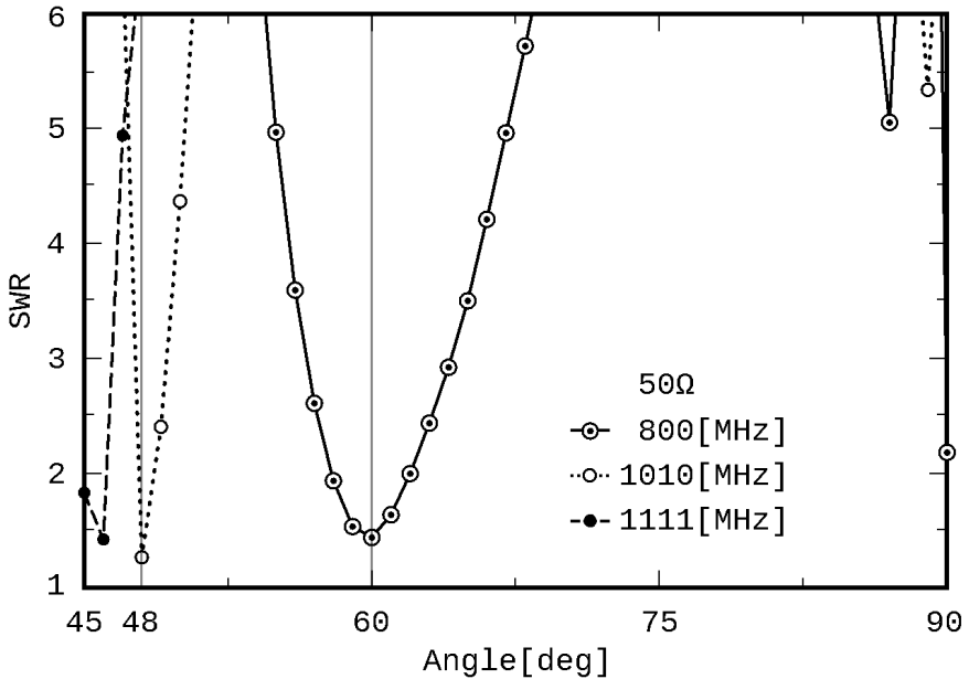
Fig. 16: SWR for 50 [ \Omega ] characteristic impedance
