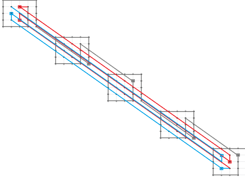
Figure 3. The rectangular spiral pattern for n = 5 (in red and light blue). This is the shortest path (length = n^3 - 1 units), no crossing lines, no points visited twice, h_u(5) = 41 .
