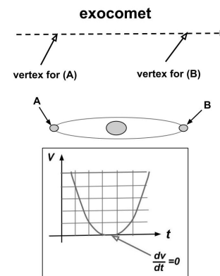
FIG. 13. Parallax experiment, to validate TPB in exocomet
