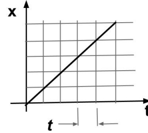
FIG. 4. Actual uniform expansion (without TPB distortions)
