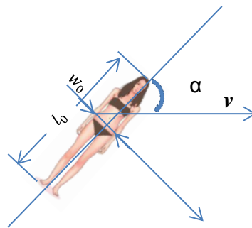
Figure 1: Alice's body rotated by an angle \alpha , relative to the direction of motion
