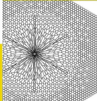
Figure 38, Quantum Dipole Repeller Gravity pushing our Galaxy. According to Quantum FFF Theory, empty space is filled with a fast oscillating lattice of massless Axion-Higgs field particles as a half base for our opposing dipole pressure Higgs-graviton gravity on earth. Now prof. Yehuda Hoffman shows us a support for this hypothesis.
