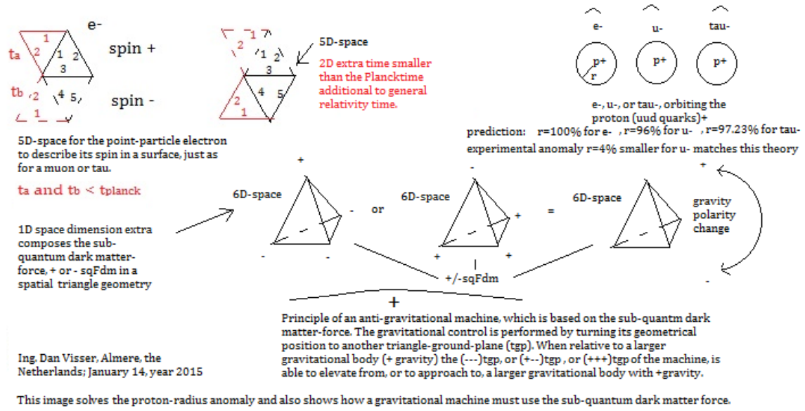
Fig. 2: Fundamental view on dimensions of dark matter and dark matter force, which change the proton-radius when an electron, muon, or tau orbits the proton. However, additionally the principle for an anti-gravitational machine emerges based on that dark matter force.
