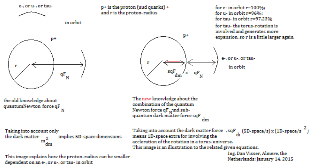
Fig. 3: The quantum Newton force ( qF_N ) is only gravitational (+). It will increase, because of a heavier mass of the muon, which is about 200 time heavier than the electron. Then the orbit will be smaller. This stronger quantum-gravity will rule the muon-hydrogen atom (H) according to old knowledge of quantum Newton-force. However, as a consequence, and according to the new knowledge of the sub-quantum dark matter force ( \pm sqF_{dm} ) being involved, equation(4) implies not only the + characteristic is smaller, but also the negative characteristic. Hence the proton simultaneously feels less negative dark matter force. And less negative dark matter force means less expansion of the proton-radius. Thus the proton-radius will become smaller. A 4% smaller
