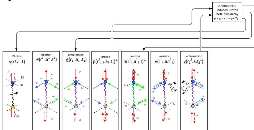
Figure 3: Proposed NLHV structures of the inputs and outputs to the antineutrino-induced \beta^+ decay.
