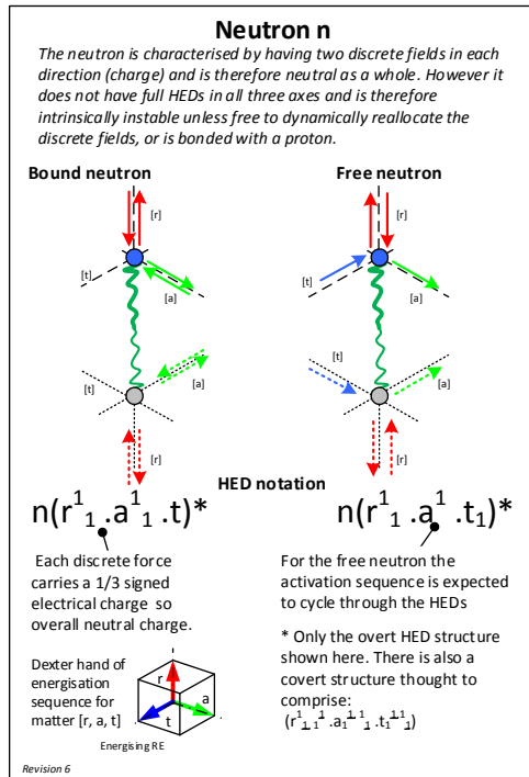
Figure 1: Proposed internal and external (discrete force) structures of the neutron. From [13], reproduced by permission.
