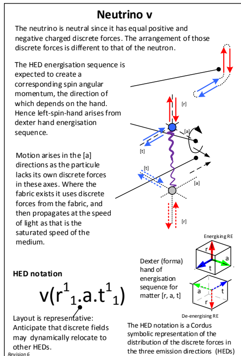
Figure 2: Predicted structure of the neutrino. From [13], reproduced by permission.
