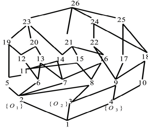
Fig. 3. Fuzzy concept lattice for the context shown in Table 5.
