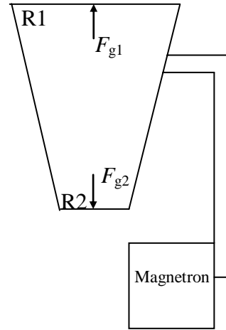
Fig. 1 – Schematic diagram of Sawyer's thruster.
