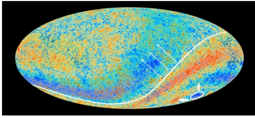
Fig 7: CMB Map by ESA's PLANK.
