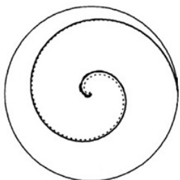
Rest Mass Particle in Single Frame
