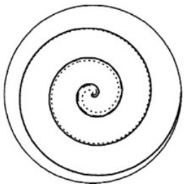
Accelerated Particle in Single Frame
