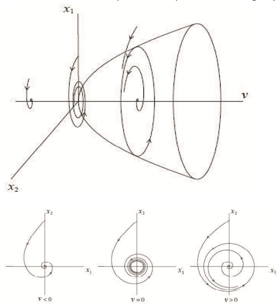
Fig 5: Supercritical Hopf Bifurcation in stable state when operating value of parameter is less than critical value of parameter.
