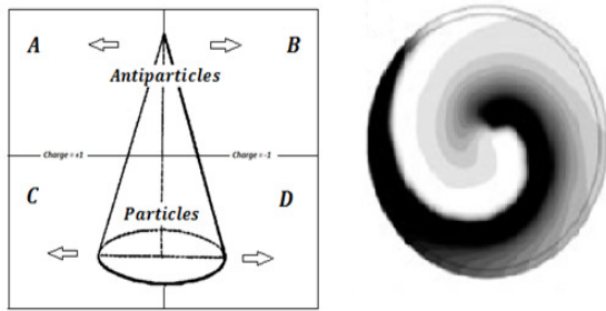
Fig 4: The orientation of curl in electromagnetically charged particle and antiparticles.
