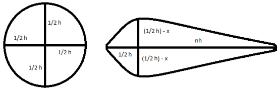
Fig 9: Fundamental unit structure of mass and extended half wave form for fermions.
