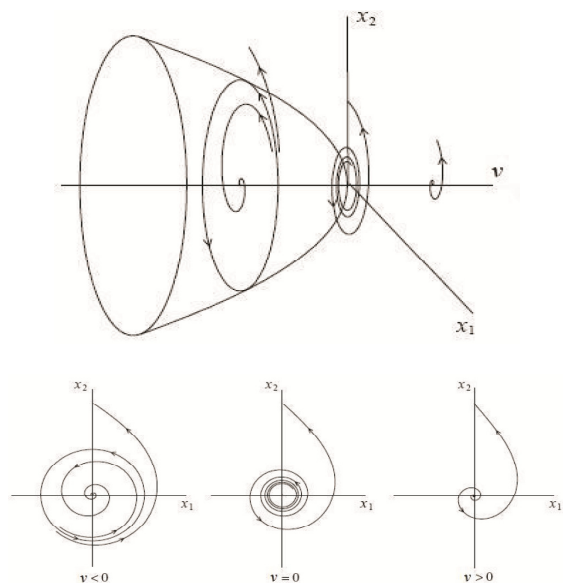
Fig 6: Supercritical Hopf Bifurcation in unstable stable state when operating value of parameter is more than critical value of parameter.
