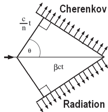
Figure 3. Geometry of Čerenkov radiation. In the figure, v is the velocity of the particle (arrow), \beta is v/c and n is the refractive index of the medium. The arrows are the direction of Čerenkov radiation so that \cos \theta = 1/n\beta .
