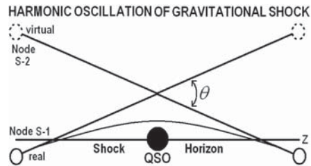
Figure 8. Schema of the primary postulate for a gravitational 'light boom' with harmonic shock cascades.
