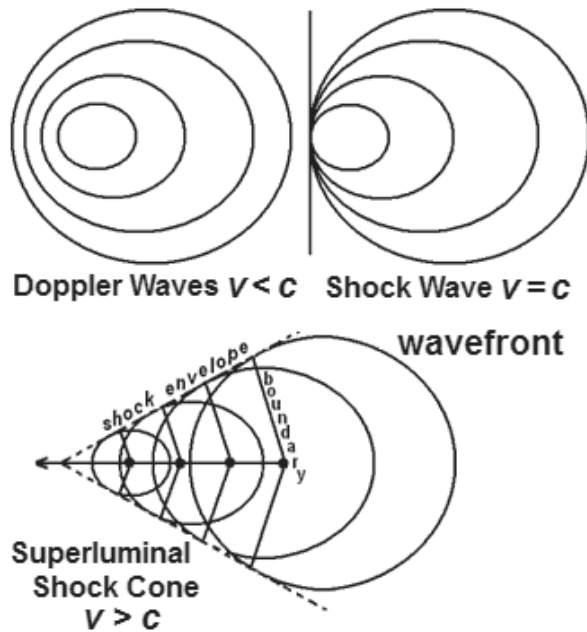
Figure 2. a) Depiction of Doppler waves, b) luminal Shock Waves and c) superluminal shock wave.
