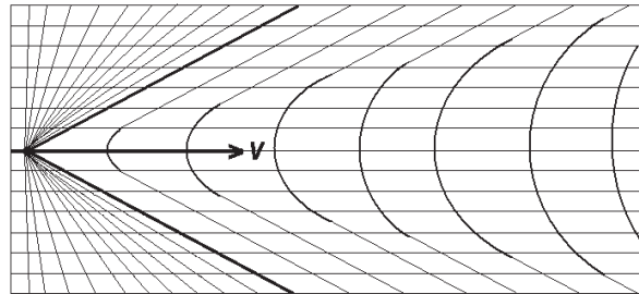
Figure 1. Wave front of a Doppler redshift for Z = \sim .85 c .
