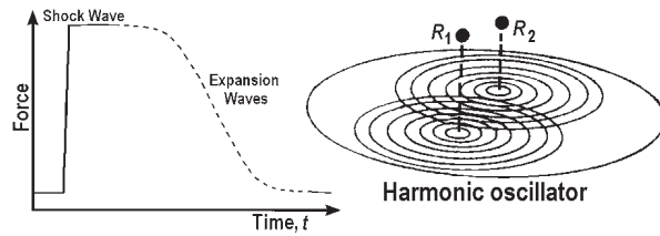
Figure 4. a) General shape of a simple shock wave. b) Harmonic oscillator effect. If superluminal shocks oscillate harmonically because of the putative dual nature of geometrodynamics they may undergo constructive and destructive interference creating ‘light booms’ as in Fig. 6.
