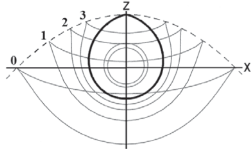
Figure 7. Select wave-fronts, a caustic or locus of cusps, when Z = 1 - x^2/4 is plotted on the dashed line of a wave envelope. Figure adapted from [60].
