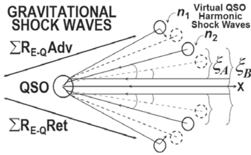
Figure 9. Elaboration of one quadrant of Fig. 8 showing a more detailed association of the oscillatory nature of the boundary conditions.
