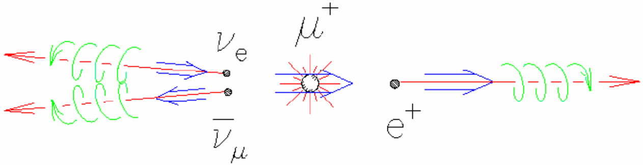
Fig. 1. Muon ( \mu^+ ) decay.
