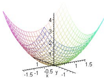
Figure 3. Bowl-shaped surfaces have positive Gauss curvature.
