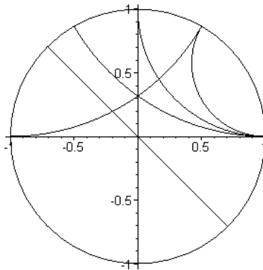
Figure 6. The Poincaré disk is a projection of the hyperbolic plane.
