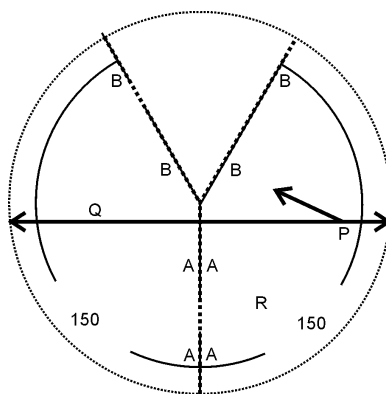
Figure 11. A cone with impulse Gauss curvature 60^\circ .
