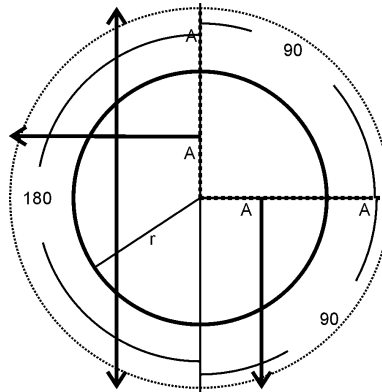
Figure 10. We can make a cone by removing a wedge.
