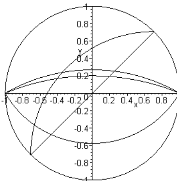
Figure 8. The image of the projective plane under stereographic projection.
