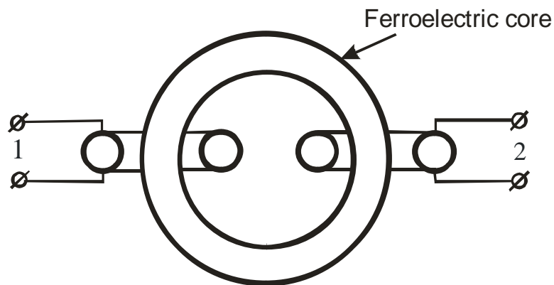
Fig. 2. Transformer with the toroidal ferroelectric core.
