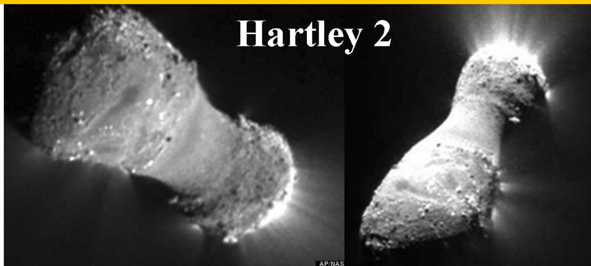
Figure: 24, both comets more in detail.
