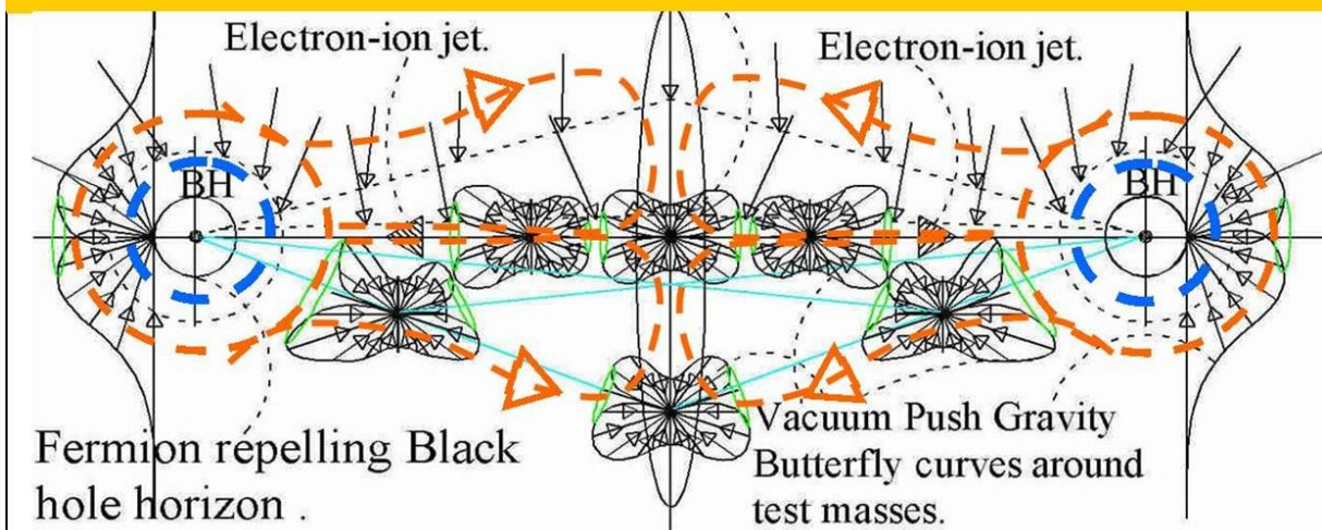
Figure: 25, Comet 67P C-G, with electrical model of the dual dark matter black hole system with O H Hydroxyl and water ice production.
