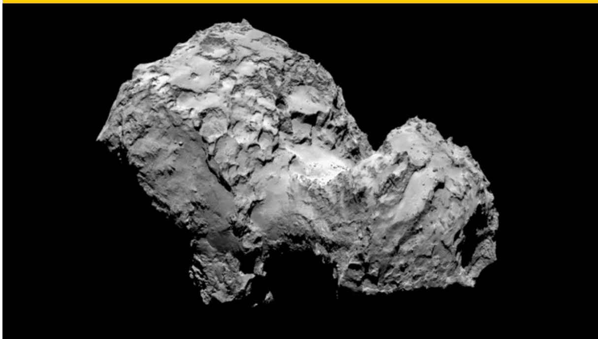
Figure 23: Dumbbell shaped Comets, 25 Hartley and Comet 67P C-G.
