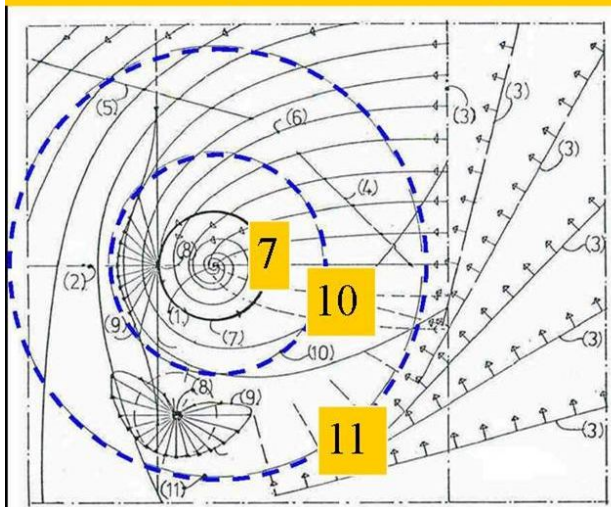
Figure: 26. Fermion repulsion principle around dark matter black holes producing water ice Comets Megacryometeors. A special example of nuclear water ice production is found in the Moon Hyperion, which is assumed to be a former Comet, left alone by its Black Hole energy source.
