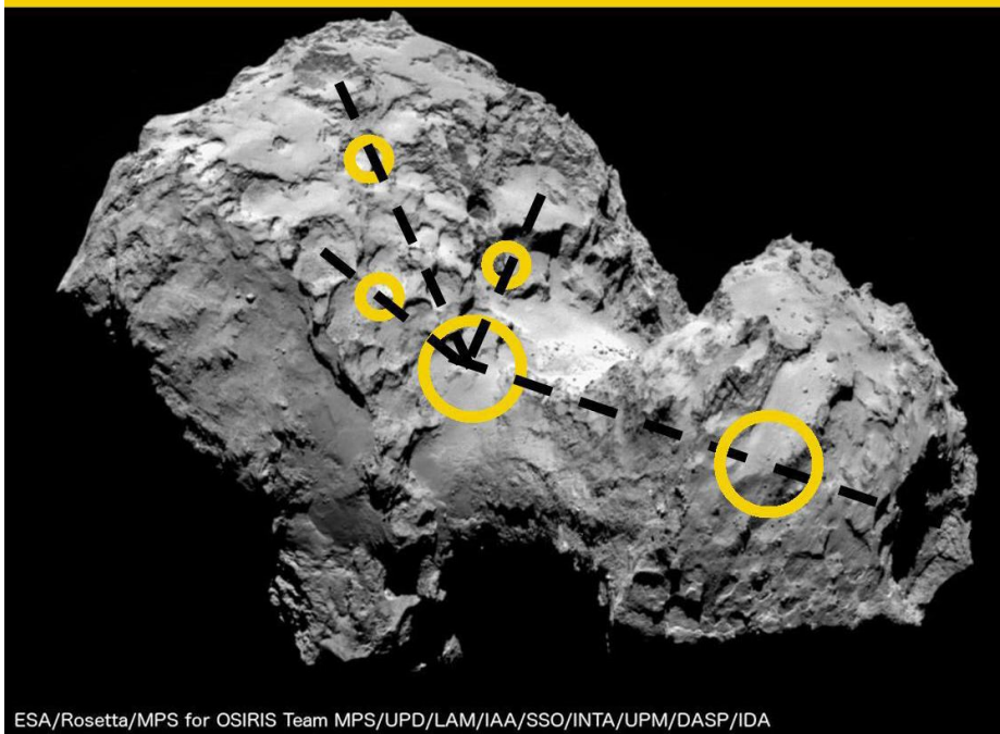
Figure: 27, Proposal for the origin of circular craters at Comet 67p C-G.
