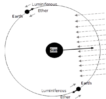
Fig. 2 The expected effect of the luminiferous ether on the speed of light
