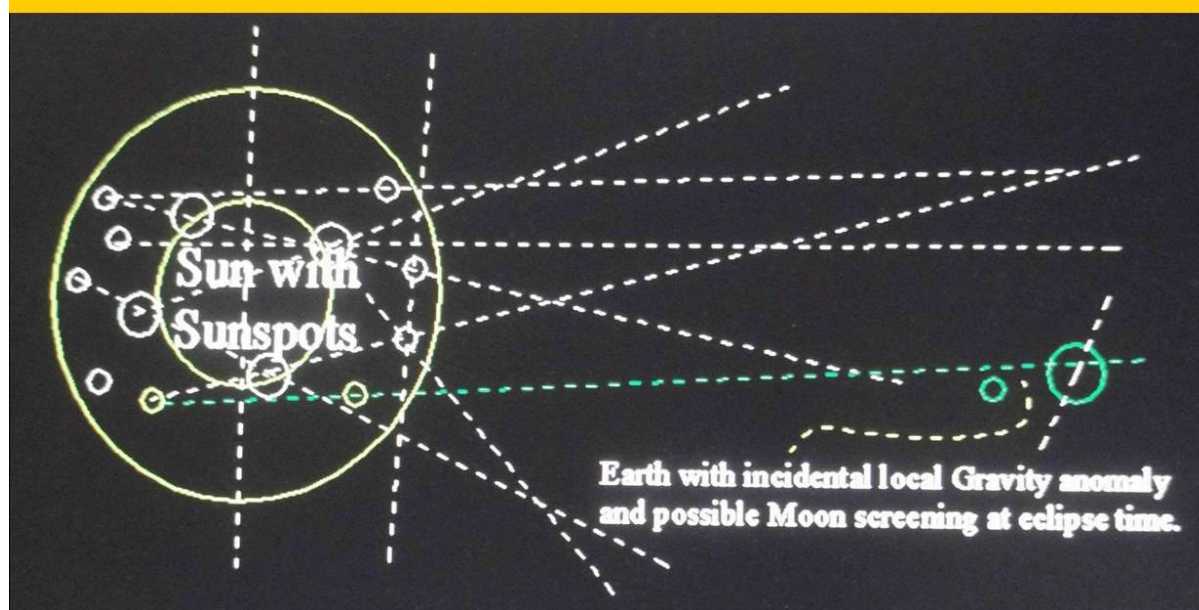
Figure: 1, Solar anomalous lensing differences and angle shift of background stars, by Solar pencil shaped gravity increase in space.
