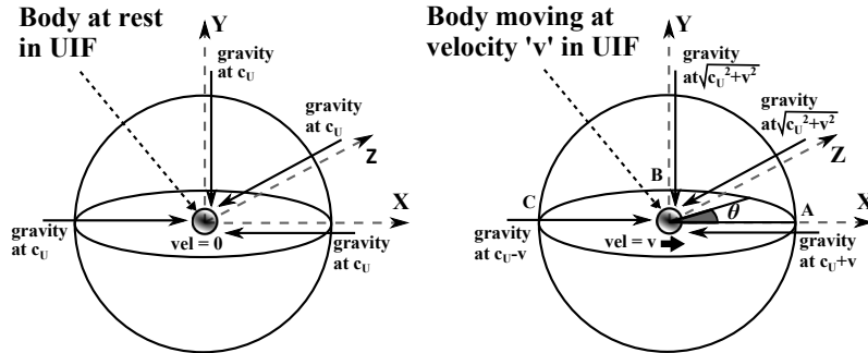
Figure 2: Universe background gravitational potential change with velocity.
