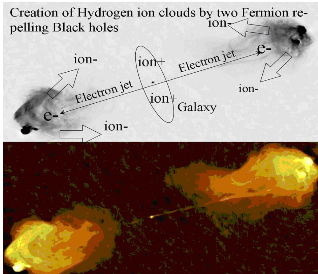
Figure 6 Cygnus A equipped with dual hotspots with gas production and electron jet including Birkeland currents and gas transportation by Alfvén circuits.
