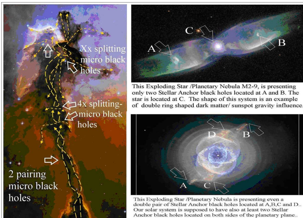
Figure 4, Examples of stellar anchor black holes and the formation of Herbig Haro systems inside the Spire nebula (left) by migrating and pairing black hole systems.
