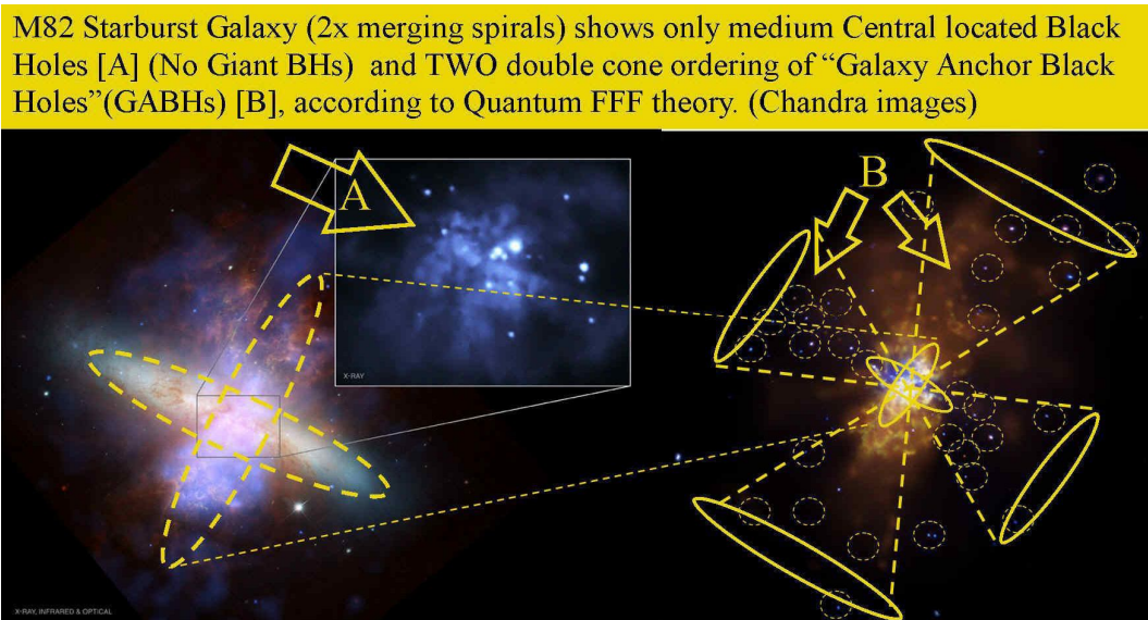
Figure 16, M82 Starburst Galaxy with a complex galaxy anchor black hole system
