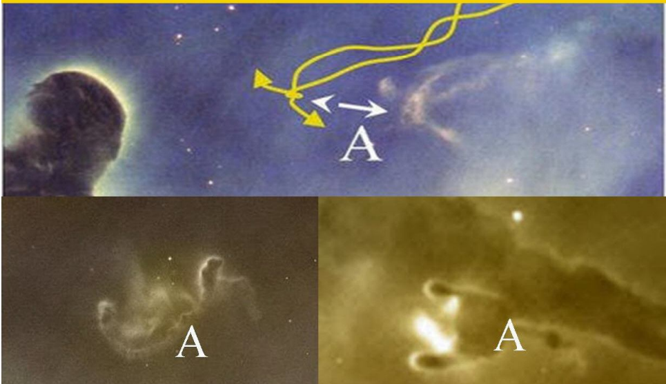
Figure 10, Three examples of ZPE accelerated Black Holes, plasma producing, pairing and splitting inside the Carina nebula.
