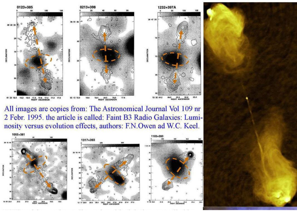
Figure 11, Cygnus A (right) is one of the best examples of Birkeland current driven gas concentration between dark matter Galaxy Anchor Black Holes (GaBHs) . Even in the early universe these dumbbell structures have been found like the “Faint B3 Radio Galaxies” (Owen and Keel)
