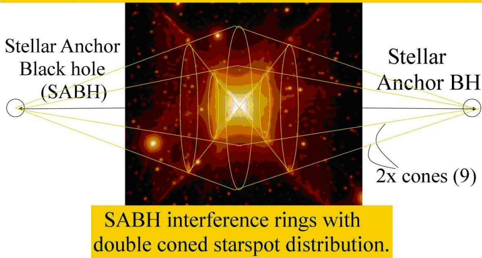
Figure 5, Star spots are supposed to be micro black holes and able to form interferenced double cone patterns after stellar explosion. The Red Square Planetary nebula MWC922, equipped with double cone structure of expelled material including trailing starspots (Micro Black Holes). There are FOUR cones of interferences observed, originated by the two Stellar Anchor Black holes (SABHs). These four cones seem to interfere with the TWO cones of expelled material of the star, leading to FOUR rings of interference.
