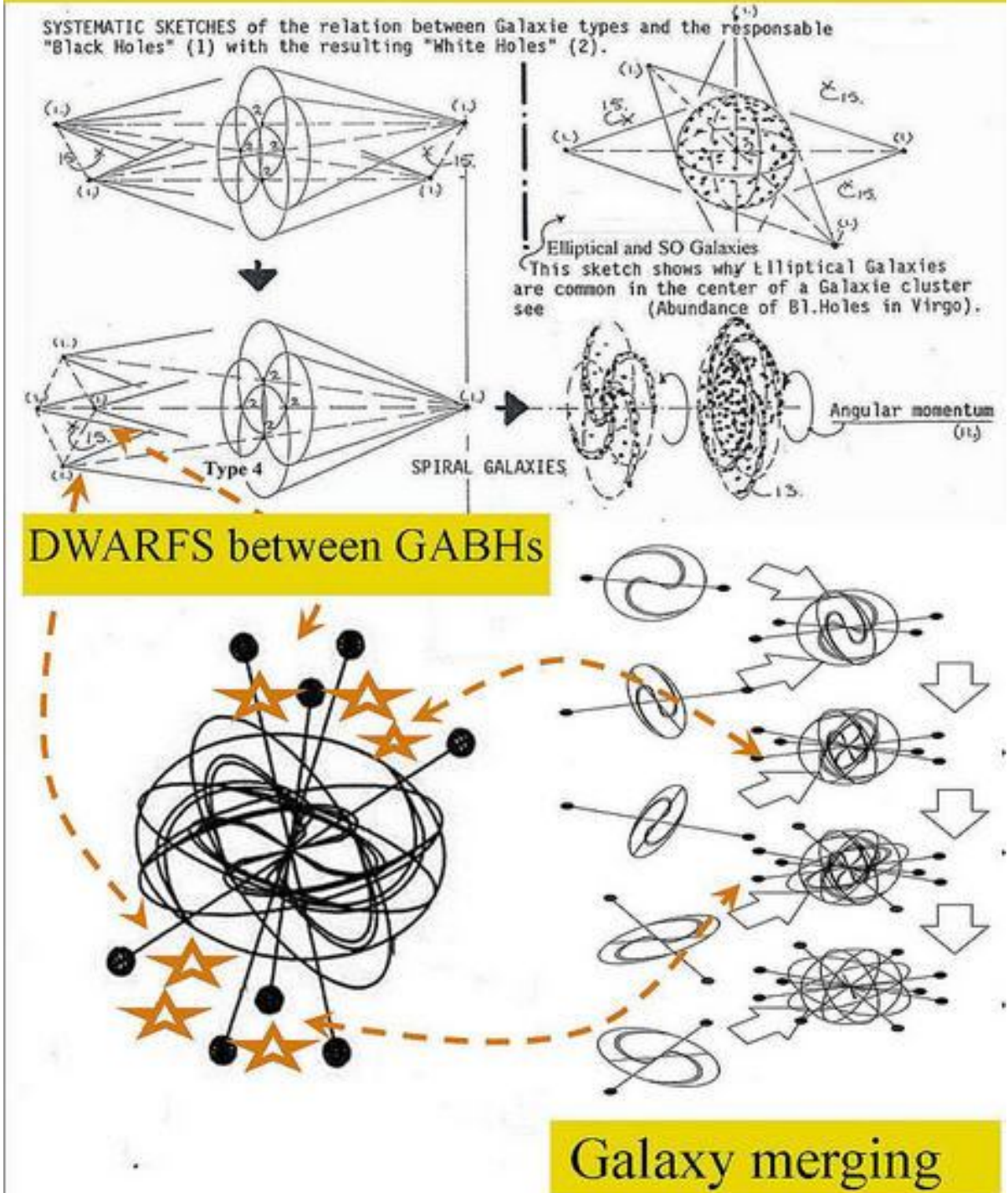
Figure 18, Dwarf galaxy formation between GABHs ( Galaxy Anchor black Holes ). TWO GABHs are able to form spiral galaxies in between. After merging with other spirals they can form more complex galaxies ( even elliptical galaxies ) , surrounded by more complex systems of GABHs. In between these GABHs there will automatically form DWARF GALAXIES.
