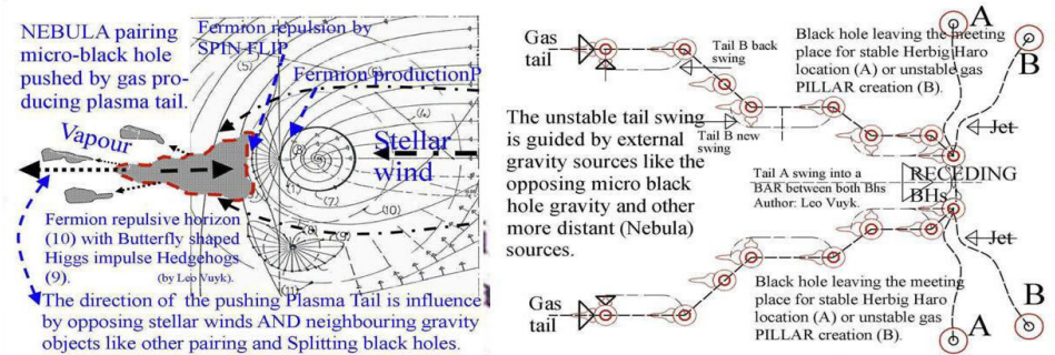
Several accelerating pairing and receding micro black holes, as the start of HH objects, in the Carina nebula, with temporary meeting place (A) and ionised plasma tail.(Quantum-FFF Theory)
