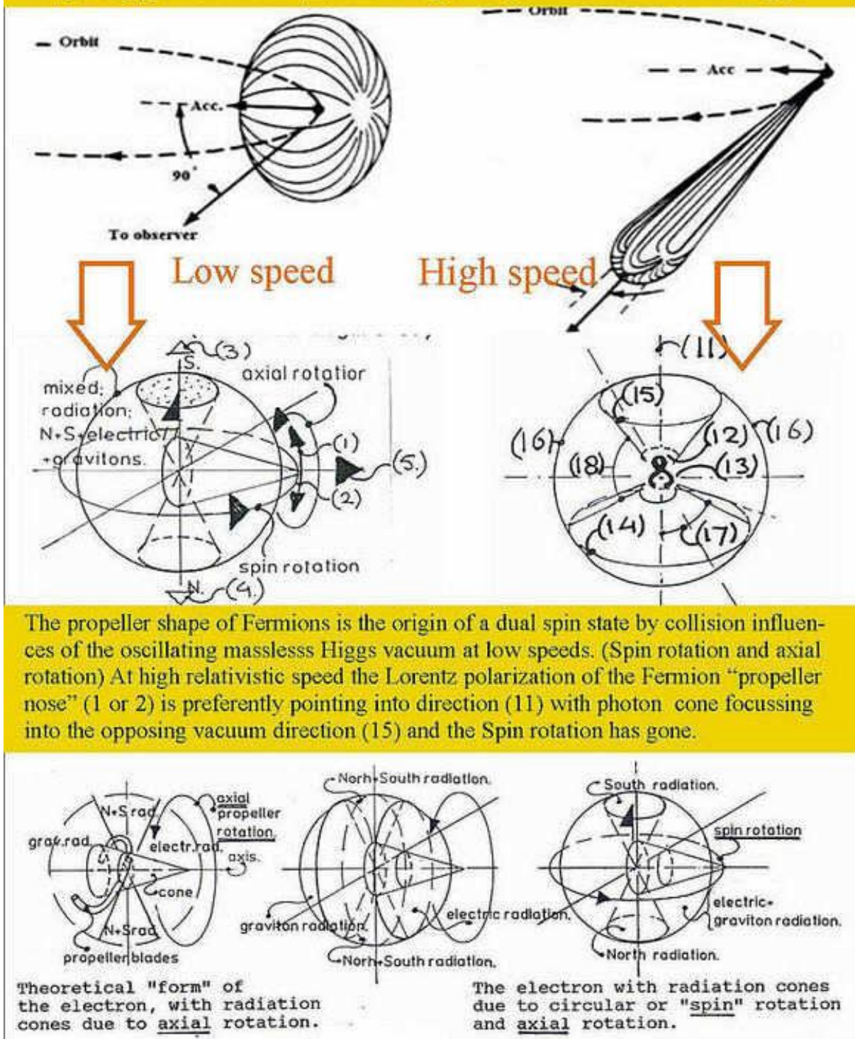
Figure 21, The polarisation of the double spinning propeller shape of fermions is the origin of all radiation differences.
