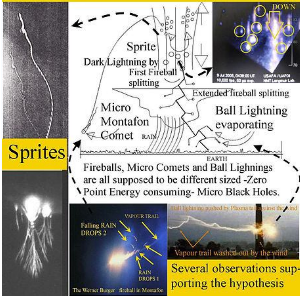
Figure: 26, Production by electro magnetic interference of the Higgs Aether into micro Black Holes or Quantum Knots as the base for Ball Lightning, Micro Comets or Sprites and Elve phenomena.
