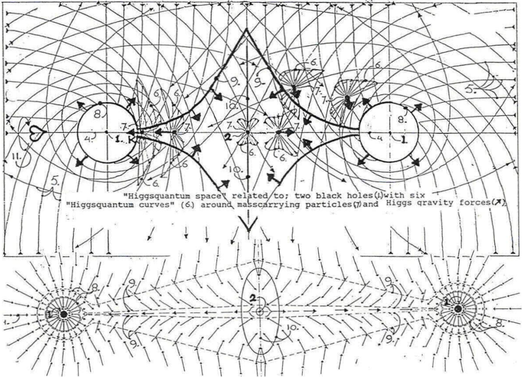
Figure 2, impression of the Higgs Vacuum structure around a set of two Black holes, as is found to be present around some Planetary nebula, early Galaxies and Herbig Haro objects. The negative charged particle jets is the result of the Black hole based electric potential combined with the vacuum polarisation
