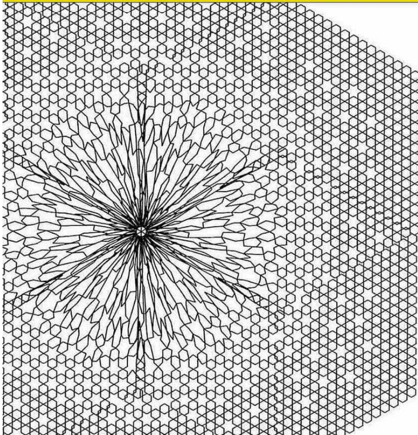
Figure 19, The Chirality and structure of the oscillating Dark Energy Higgs vacuum lattice
