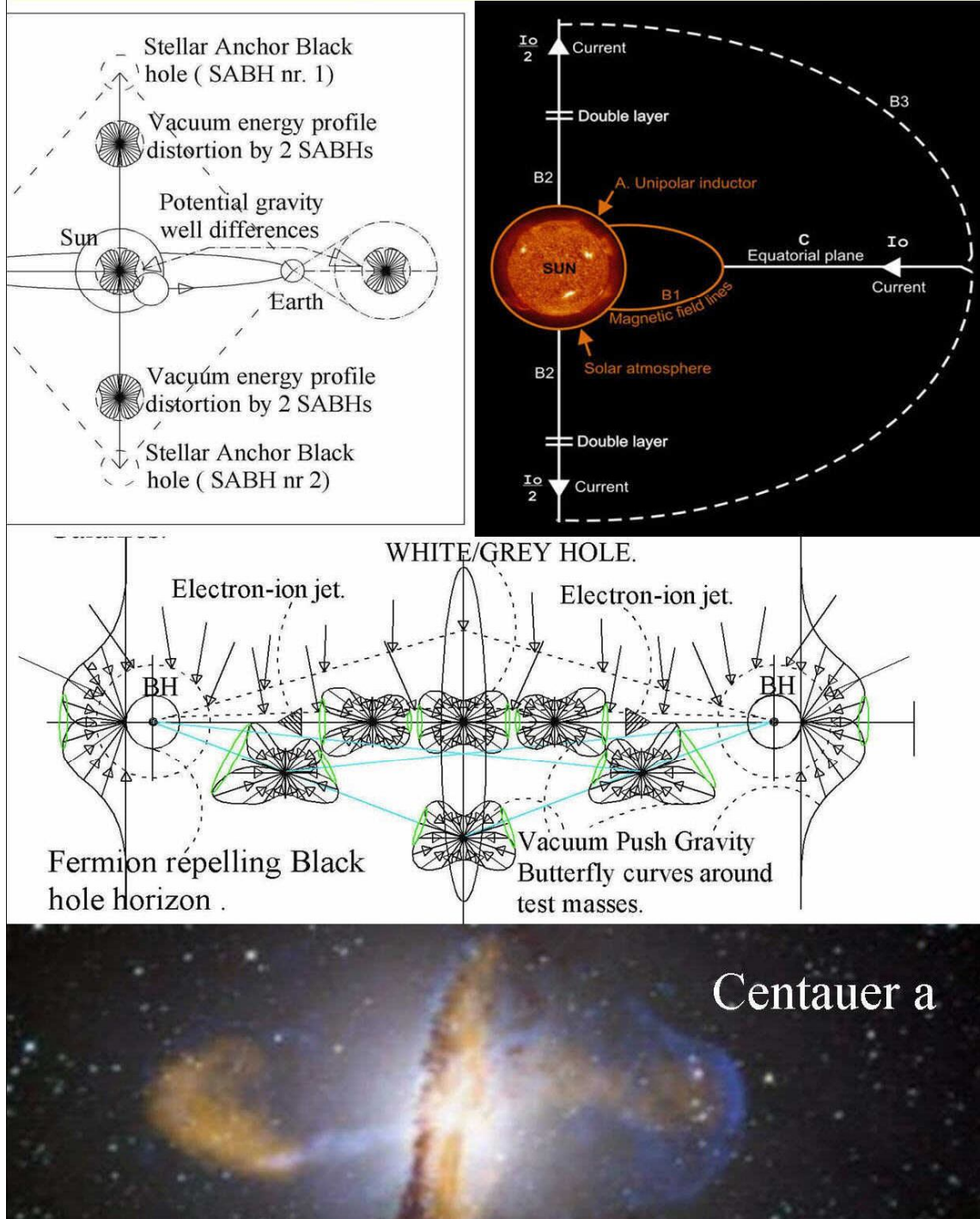
Figure 17, Birkeland current systems around stars and galaxies.
