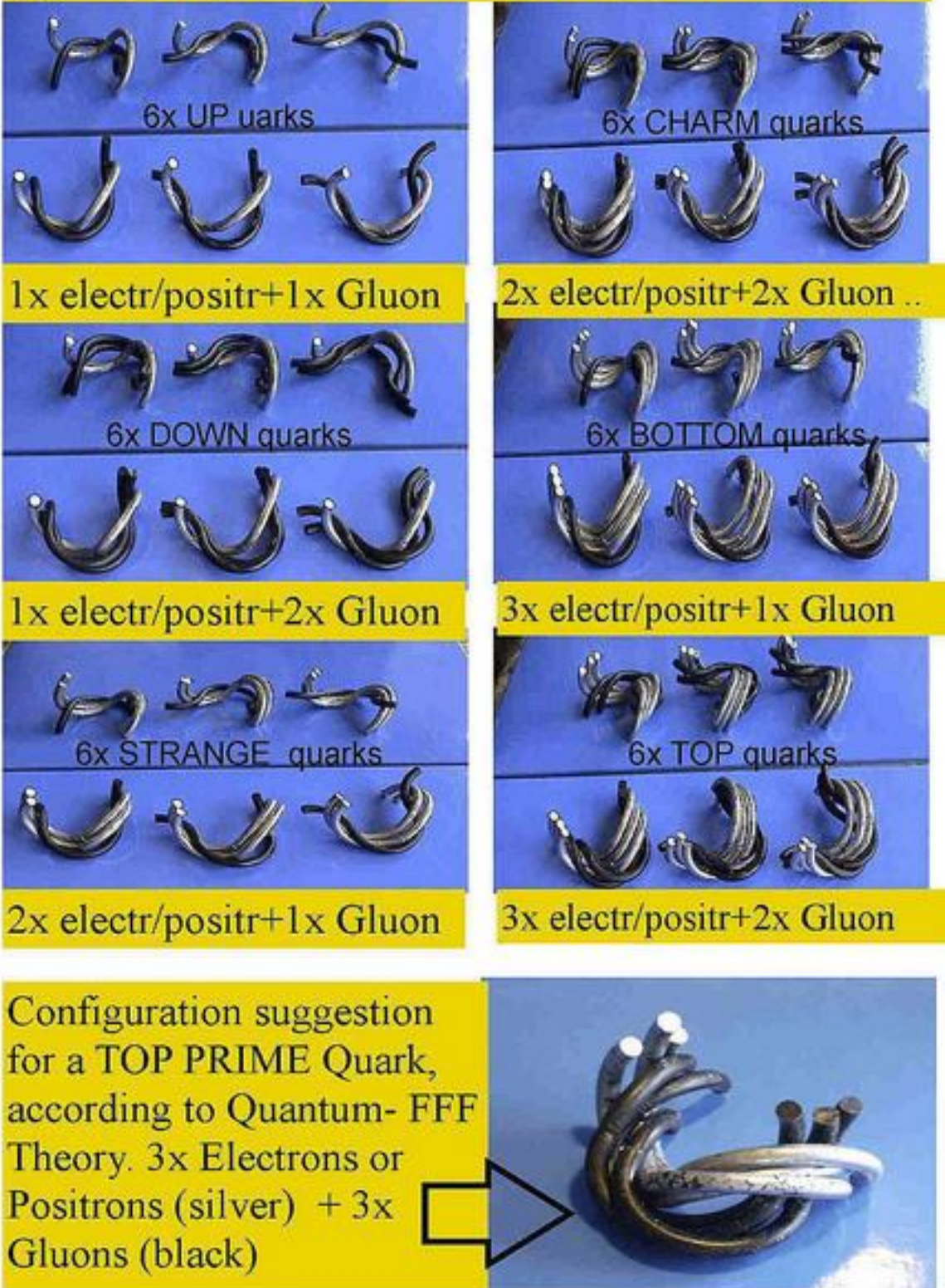
Figure 20, 5x different shaped Photon/Gluons can combine with the two propeller shapes of the electron and Positron to form all coloured (QCD) Quarks and even more!!
