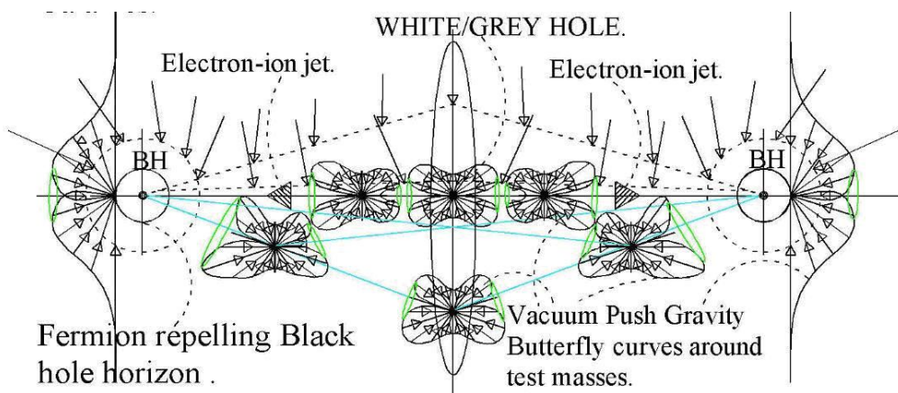
Figure 3, The same Birkeland current system as figure 2 with butterfly vector arrays at different locations around the Black holes. In the middle the vacuum has less density ( larger Planck lengths) by the absorption of the dual Black holes.
