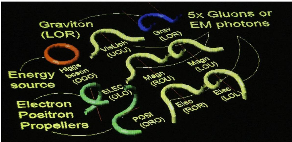
Figure 24, The particle zoo of single ELEMENTARY particles.
