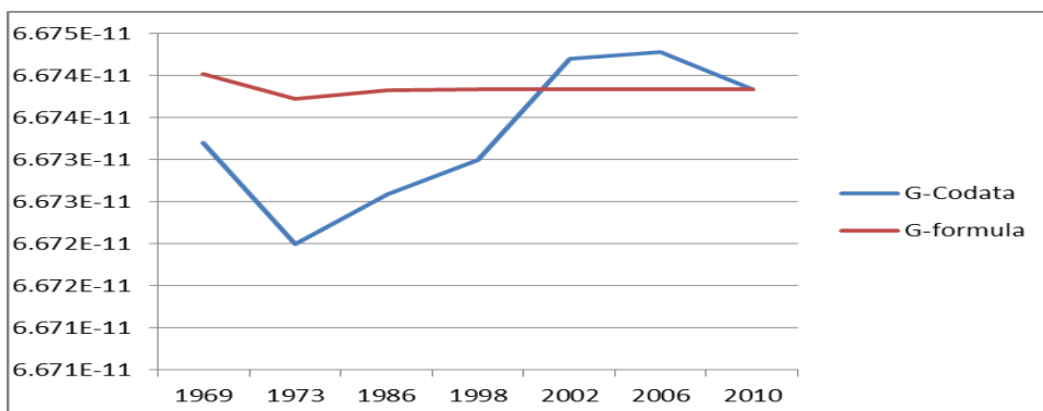
Figure 1 Universal gravitational constant – G in the 1969–2010 period CODATA values [1] and values achieved by formula (8)
